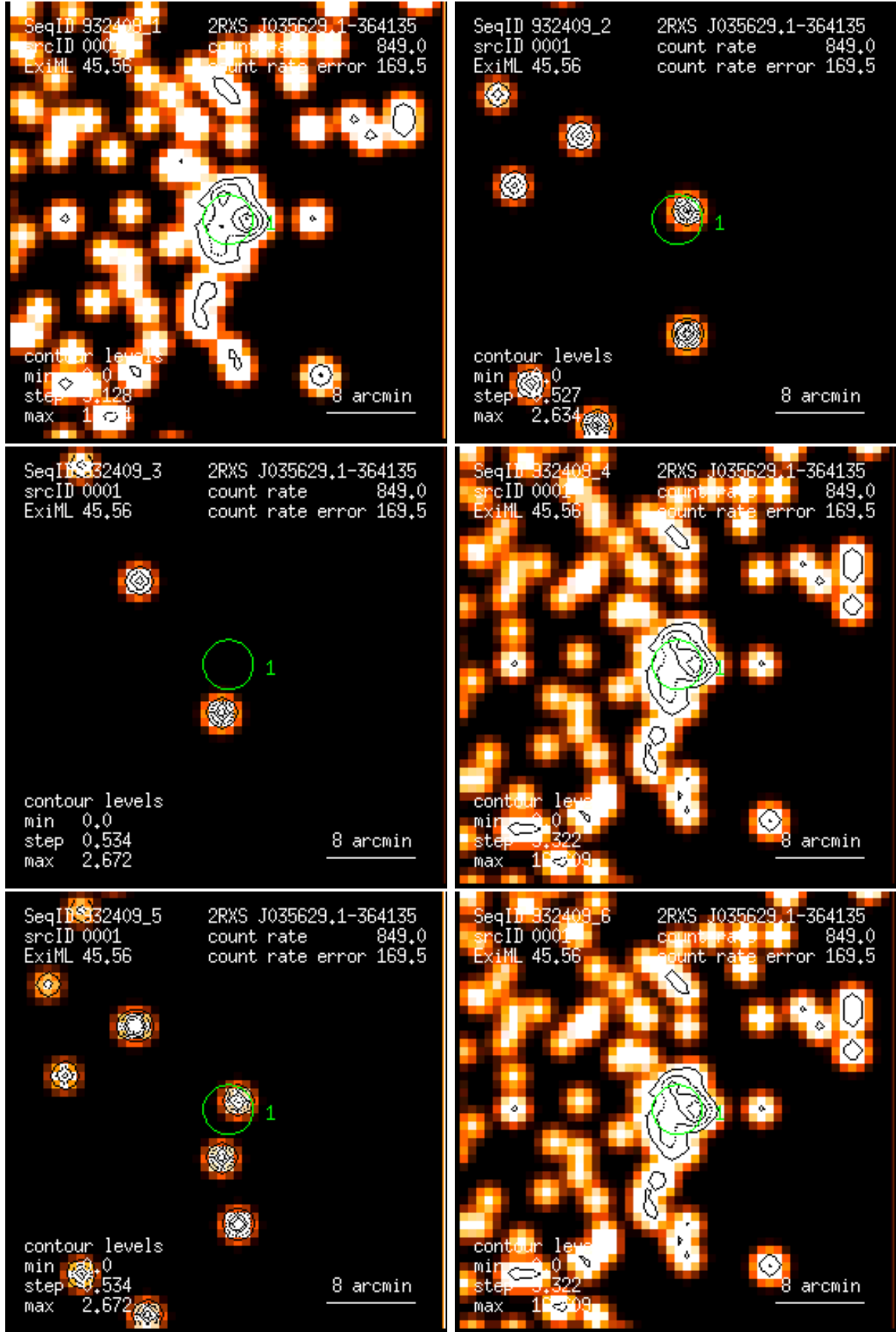
Figure 1: RASS 932409: detection 0001: band rate images, Gaussian filter: (1) PSPC channels 11 – 41, (2) 52 – 90, (3) 91 – 201, (4) 11 – 235, (5) 52 – 201, (6) 11 – 201. Broad band rates in counts/ks. Band rate contour levels in counts/ks/arcmin 2 .
