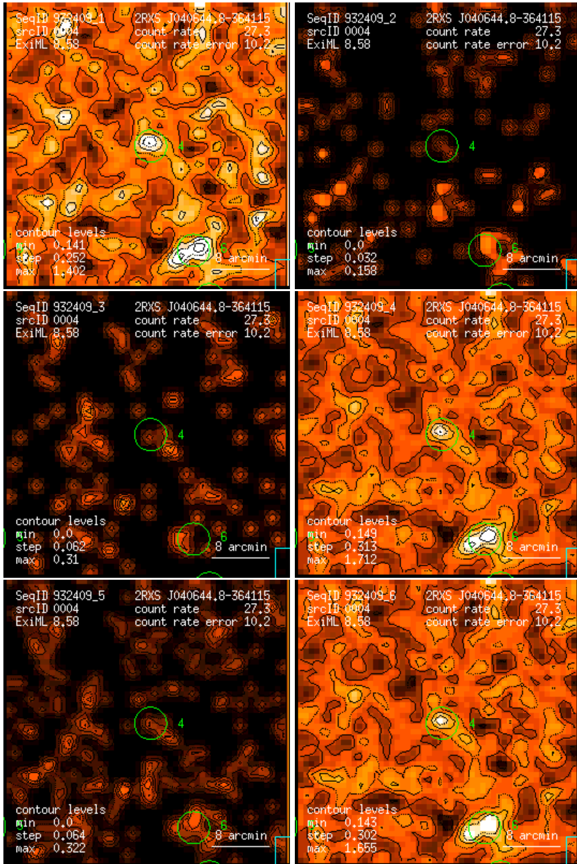
Figure 4: RASS 932409: detection 0004: band rate images, Gaussian filter: (1) PSPC channels 11 – 41, (2) 52 – 90, (3) 91 – 201, (4) 11 – 235, (5) 52 – 201, (6) 11 – 201. Broad band rates in counts/ks. Band rate contour levels in counts/ks/arcmin 2 .
