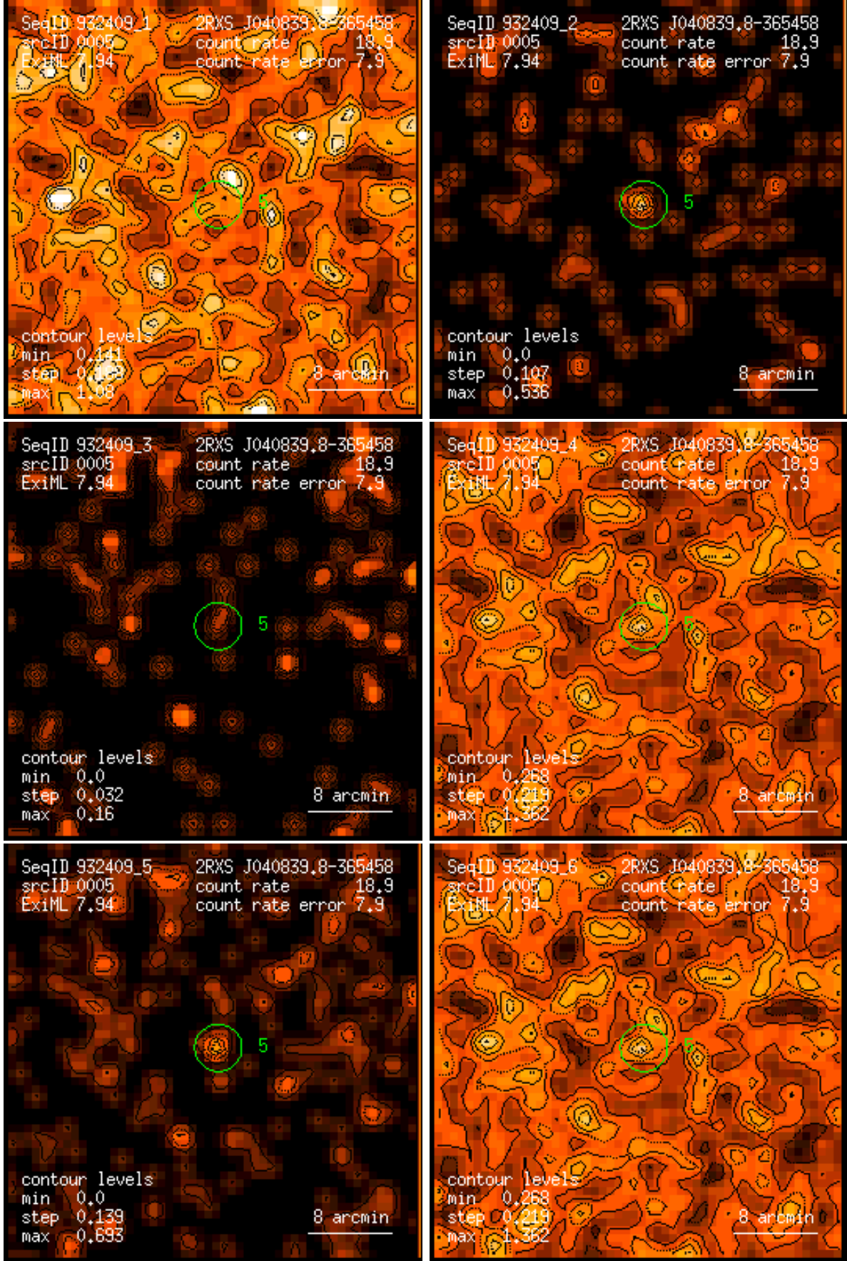
Figure 5: RASS 932409: detection 0005: band rate images, Gaussian filter: (1) PSPC channels 11 – 41, (2) 52 – 90, (3) 91 – 201, (4) 11 – 235, (5) 52 – 201, (6) 11 – 201. Broad band rates in counts/ks. Band rate contour levels in counts/ks/arcmin 2 .
