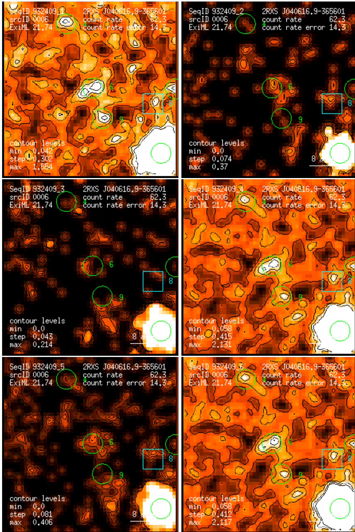
Figure 6: RASS 932409: detection 0006: band rate images, Gaussian filter: (1) PSPC channels 11 – 41, (2) 52 – 90, (3) 91 – 201, (4) 11 – 235, (5) 52 – 201, (6) 11 – 201. Broad band rates in counts/ks. Band rate contour levels in counts/ks/arcmin 2 .
