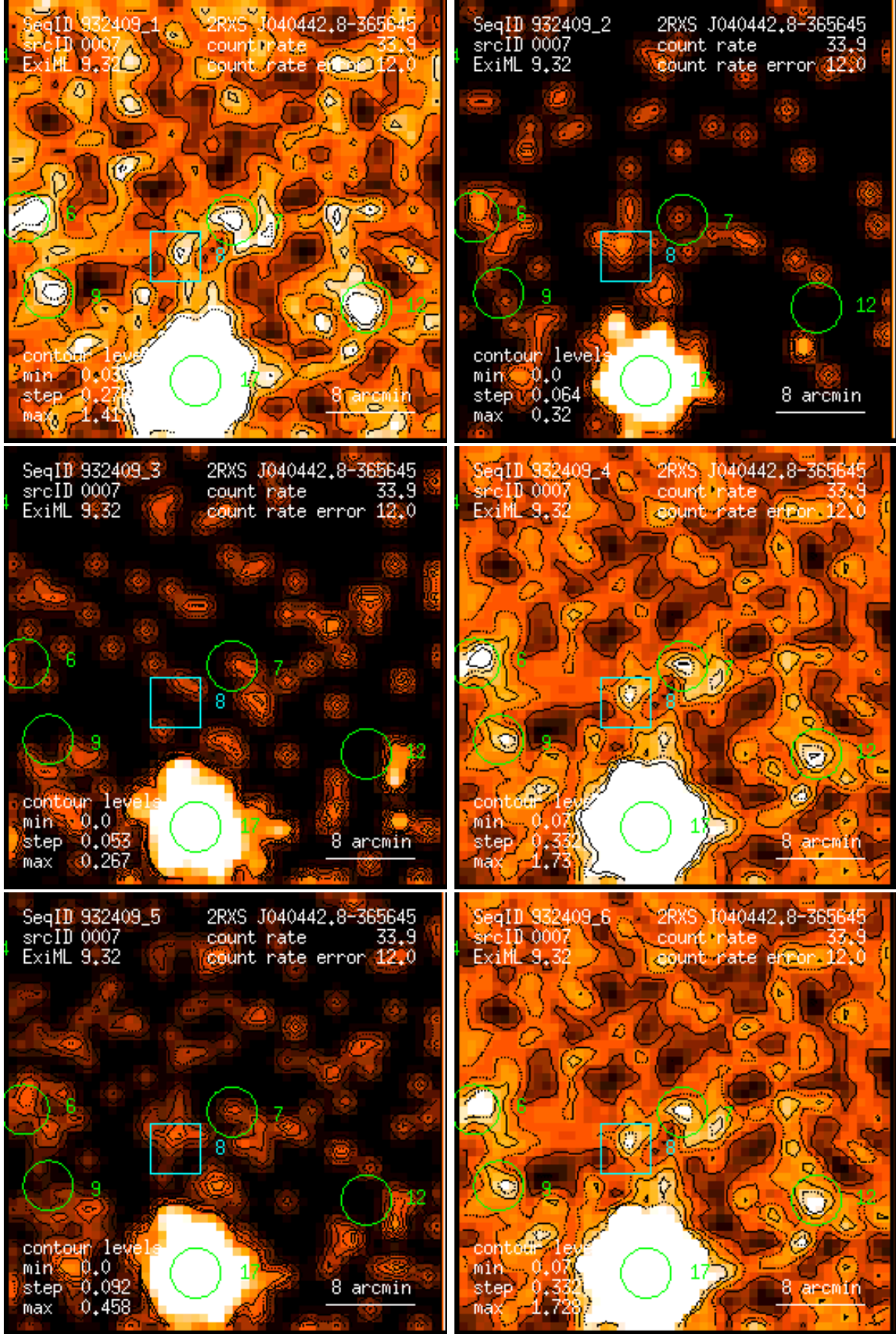
Figure 7: RASS 932409: detection 0007: band rate images, Gaussian filter: (1) PSPC channels 11 – 41, (2) 52 – 90, (3) 91 – 201, (4) 11 – 235, (5) 52 – 201, (6) 11 – 201. Broad band rates in counts/ks. Band rate contour levels in counts/ks/arcmin 2 .
