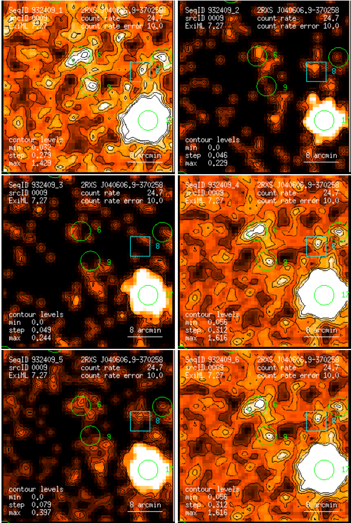
Figure 9: RASS 932409: detection 0009: band rate images, Gaussian filter: (1) PSPC channels 11 – 41, (2) 52 – 90, (3) 91 – 201, (4) 11 – 235, (5) 52 – 201, (6) 11 – 201. Broad band rates in counts/ks. Band rate contour levels in counts/ks/arcmin 2 .
