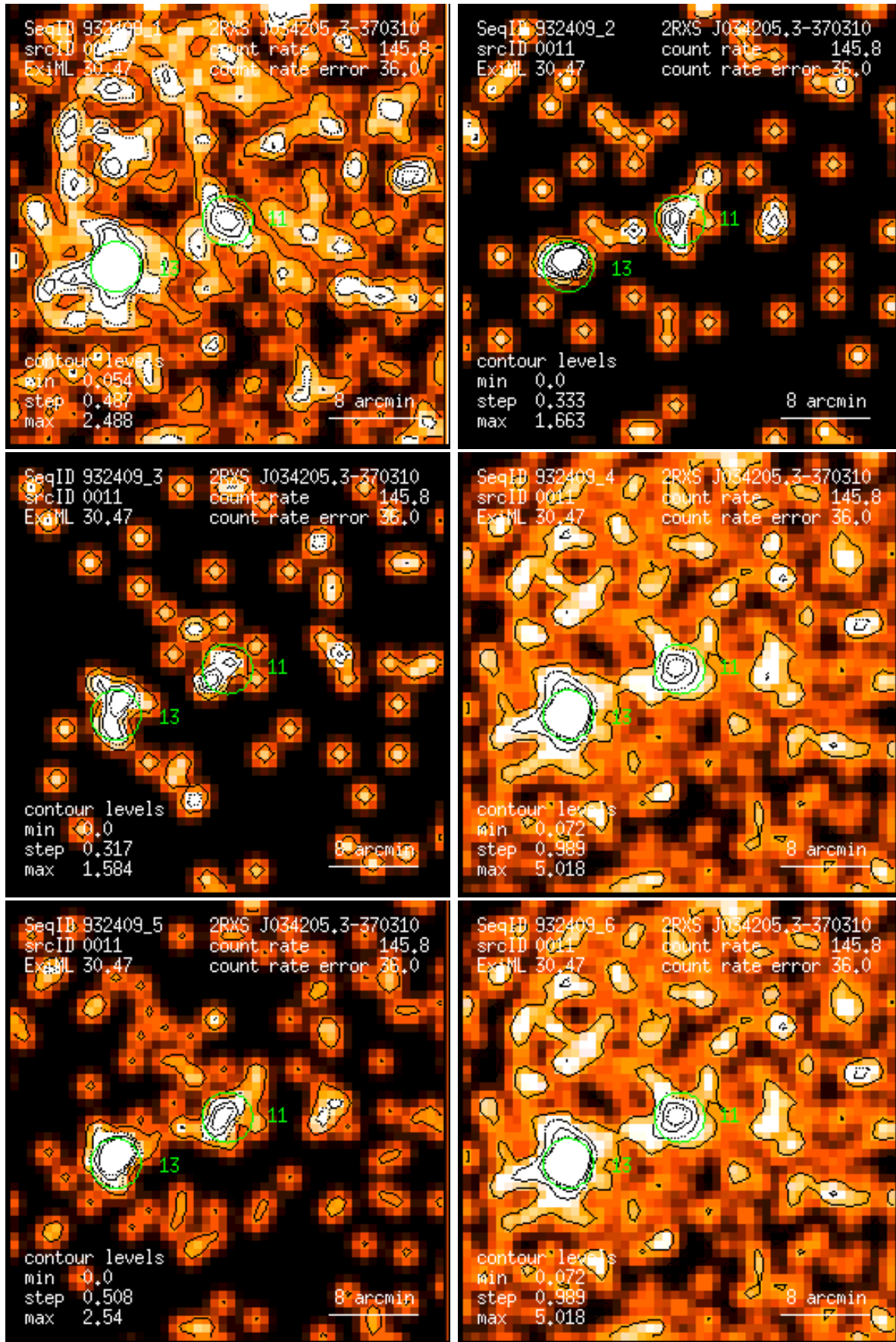
Figure 11: RASS 932409: detection 0011: band rate images, Gaussian filter: (1) PSPC channels 11 – 41, (2) 52 – 90, (3) 91 – 201, (4) 11 – 235, (5) 52 – 201, (6) 11 – 201. Broad band rates in counts/ks. Band rate contour levels in counts/ks/arcmin 2 .
