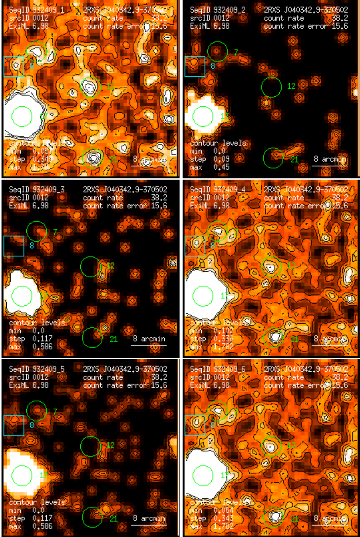
Figure 12: RASS 932409: detection 0012: band rate images, Gaussian filter: (1) PSPC channels 11 – 41, (2) 52 – 90, (3) 91 – 201, (4) 11 – 235, (5) 52 – 201, (6) 11 – 201. Broad band rates in counts/ks. Band rate contour levels in counts/ks/arcmin 2 .
