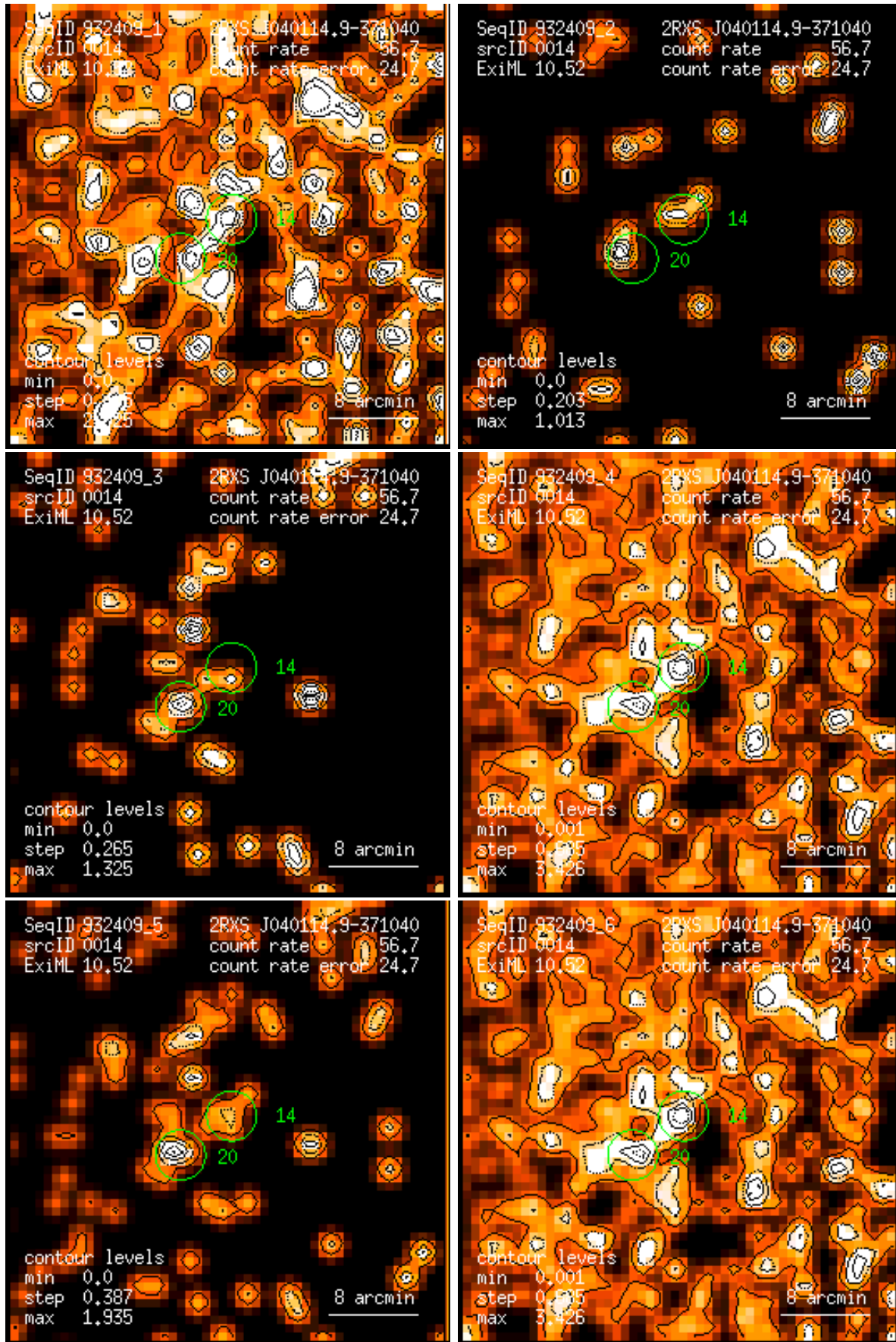
Figure 14: RASS 932409: detection 0014: band rate images, Gaussian filter: (1) PSPC channels 11 – 41, (2) 52 – 90, (3) 91 – 201, (4) 11 – 235, (5) 52 – 201, (6) 11 – 201. Broad band rates in counts/ks. Band rate contour levels in counts/ks/arcmin 2 .
