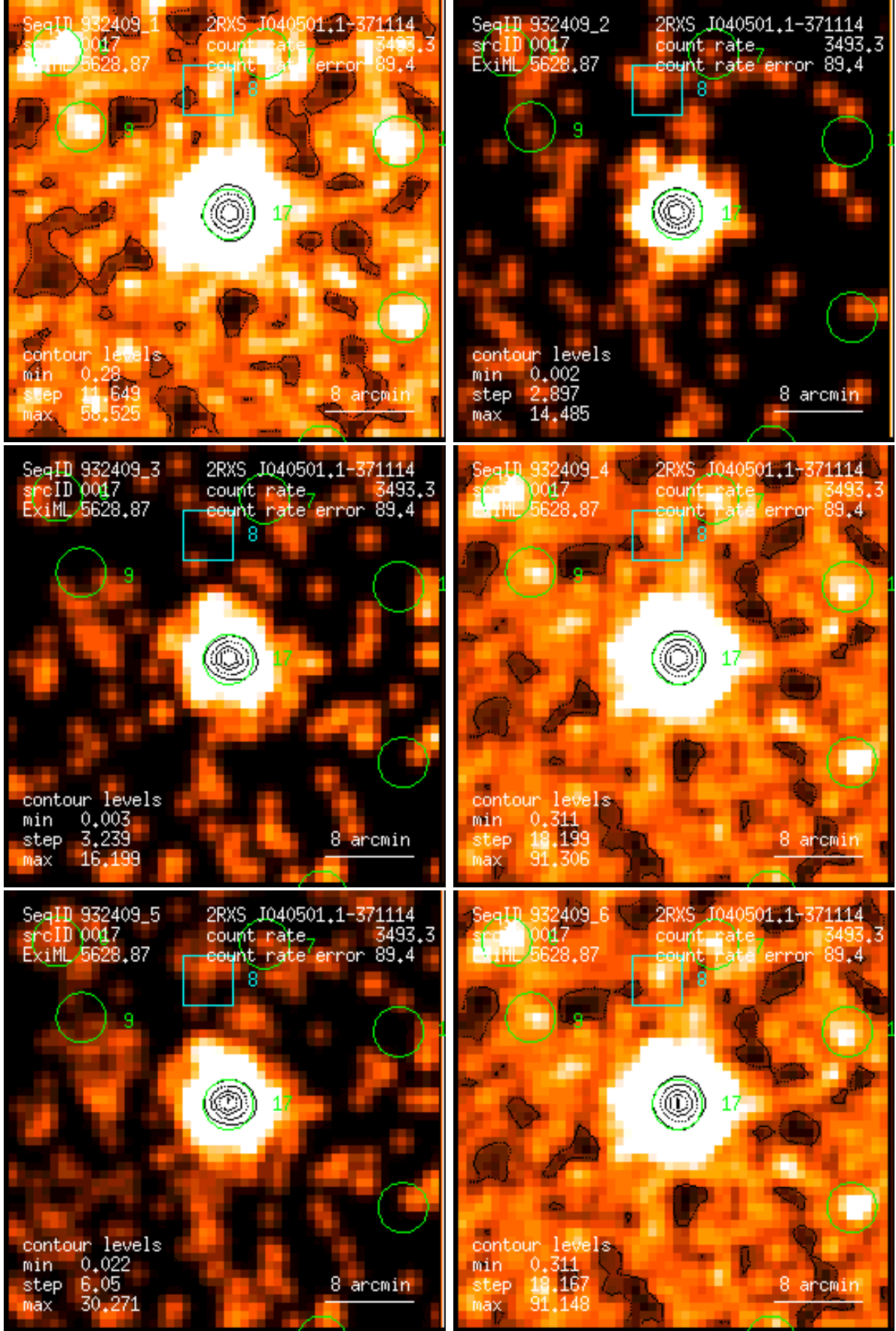
Figure 17: RASS 932409: detection 0017: band rate images, Gaussian filter: (1) PSPC channels 11 – 41, (2) 52 – 90, (3) 91 – 201, (4) 11 – 235, (5) 52 – 201, (6) 11 – 201. Broad band rates in counts/ks. Band rate contour levels in counts/ks/arcmin 2 .
