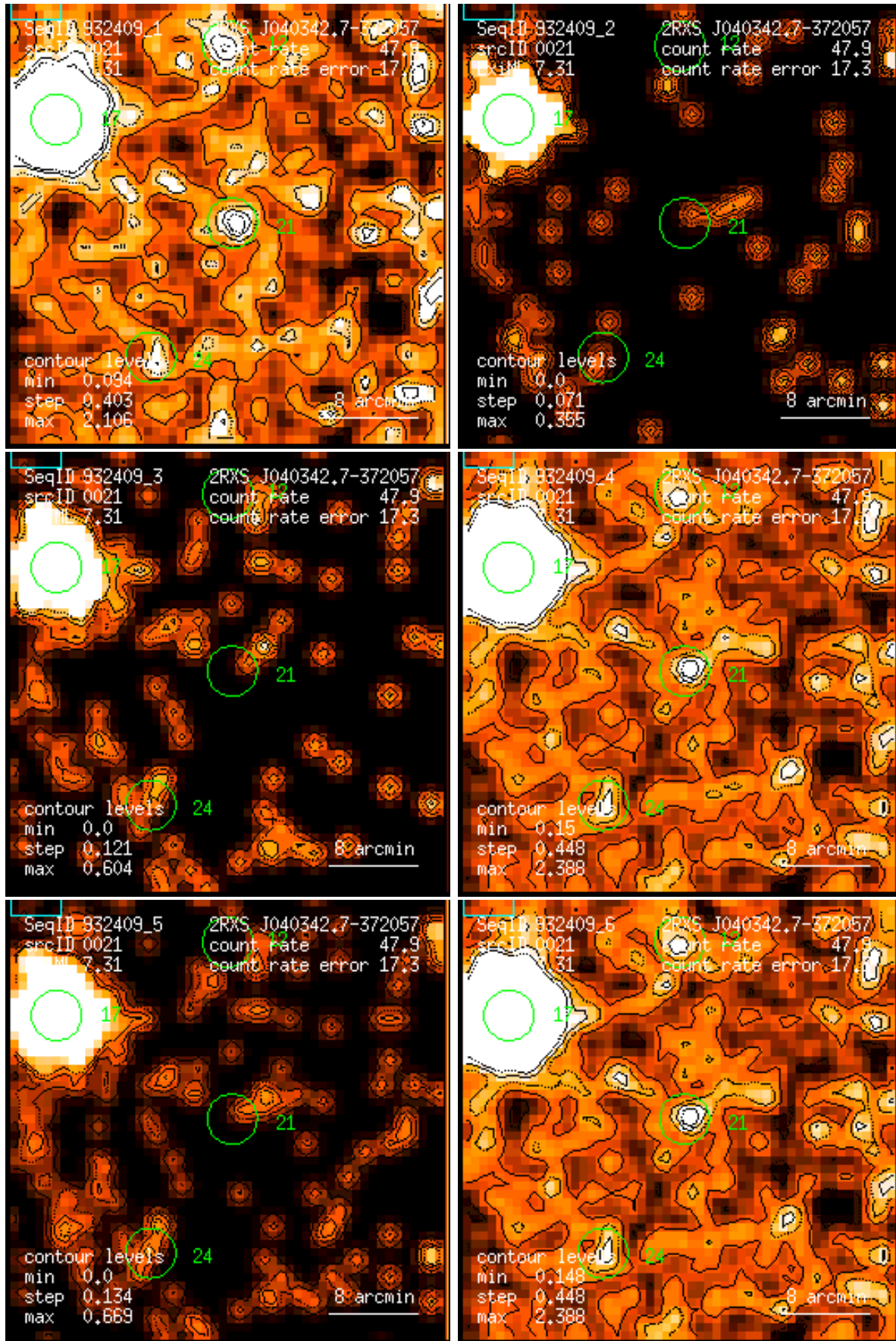
Figure 21: RASS 932409: detection 0021: band rate images, Gaussian filter: (1) PSPC channels 11 – 41, (2) 52 – 90, (3) 91 – 201, (4) 11 – 235, (5) 52 – 201, (6) 11 – 201. Broad band rates in counts/ks. Band rate contour levels in counts/ks/arcmin 2 .
