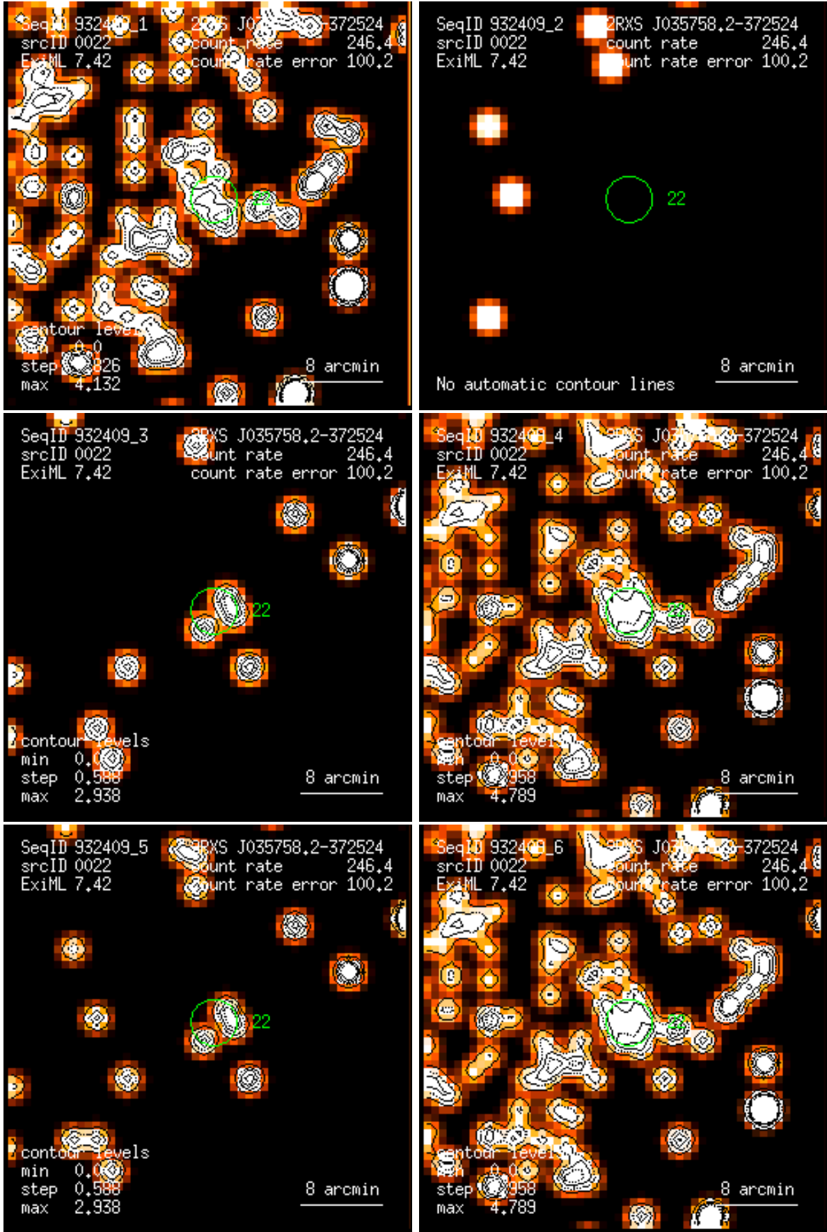
Figure 22: RASS 932409: detection 0022: band rate images, Gaussian filter: (1) PSPC channels 11 – 41, (2) 52 – 90, (3) 91 – 201, (4) 11 – 235, (5) 52 – 201, (6) 11 – 201. Broad band rates in counts/ks. Band rate contour levels in counts/ks/arcmin 2 .
