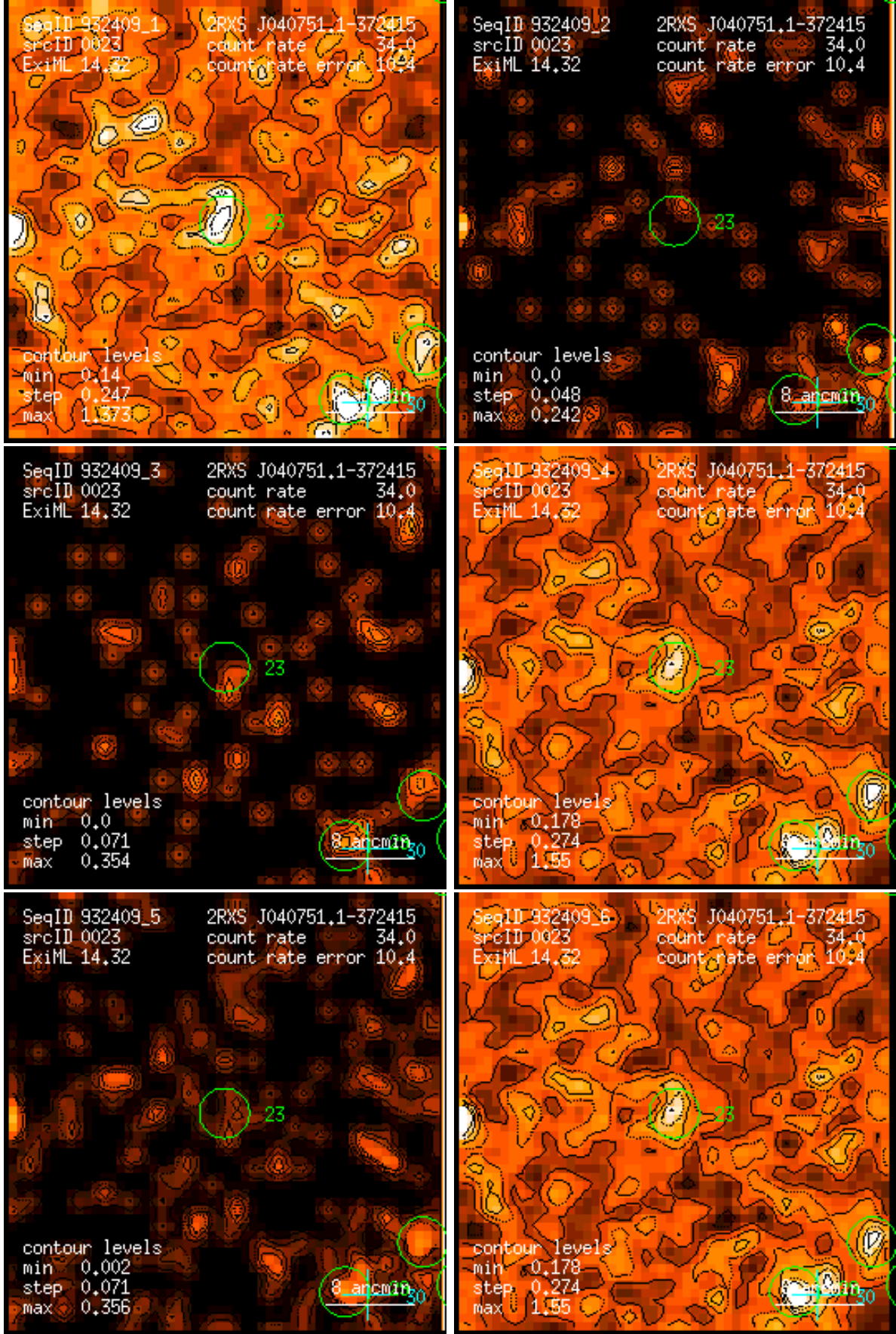
Figure 23: RASS 932409: detection 0023: band rate images, Gaussian filter: (1) PSPC channels 11 – 41, (2) 52 – 90, (3) 91 – 201, (4) 11 – 235, (5) 52 – 201, (6) 11 – 201. Broad band rates in counts/ks. Band rate contour levels in counts/ks/arcmin 2 .
