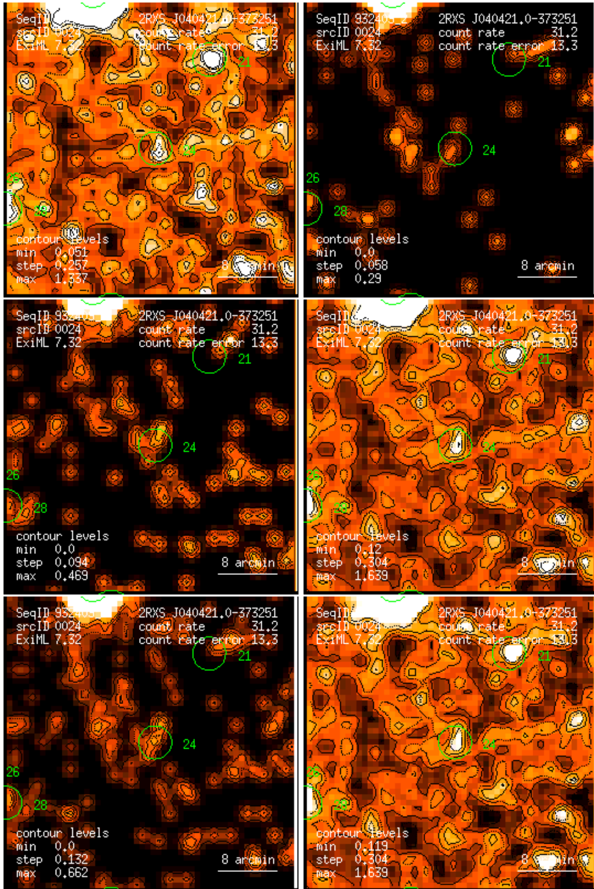
Figure 24: RASS 932409: detection 0024: band rate images, Gaussian filter: (1) PSPC channels 11 – 41, (2) 52 – 90, (3) 91 – 201, (4) 11 – 235, (5) 52 – 201, (6) 11 – 201. Broad band rates in counts/ks. Band rate contour levels in counts/ks/arcmin 2 .
