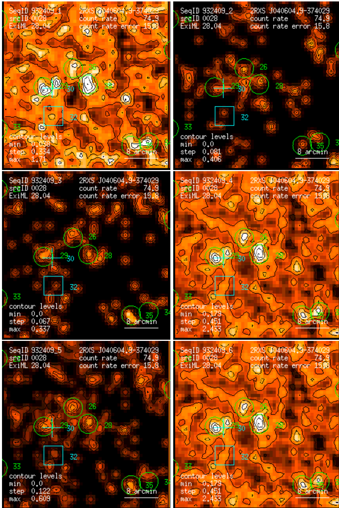
Figure 28: RASS 932409: detection 0028: band rate images, Gaussian filter: (1) PSPC channels 11 – 41, (2) 52 – 90, (3) 91 – 201, (4) 11 – 235, (5) 52 – 201, (6) 11 – 201. Broad band rates in counts/ks. Band rate contour levels in counts/ks/arcmin 2 .
