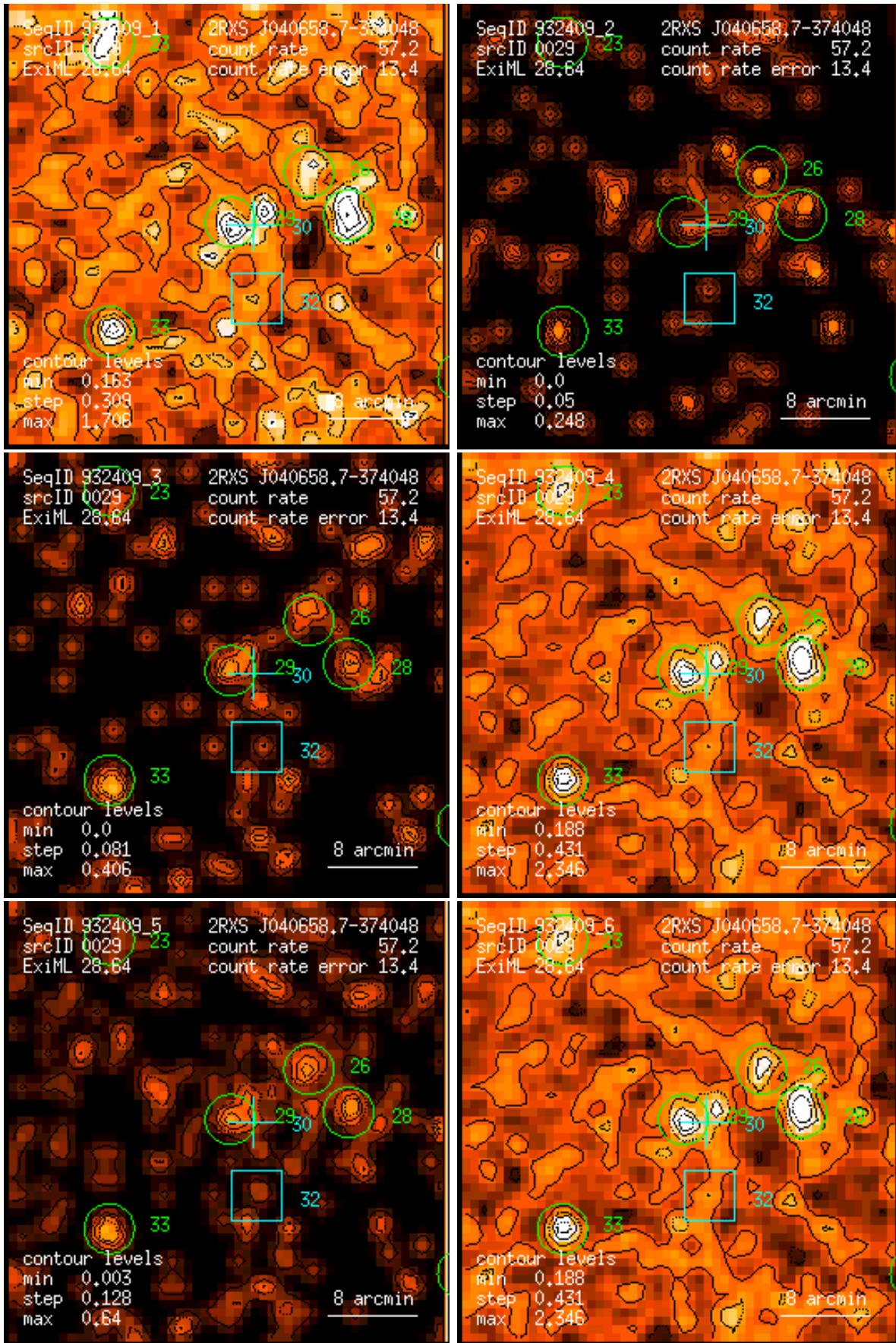
Figure 29: RASS 932409: detection 0029: band rate images, Gaussian filter: (1) PSPC channels 11 – 41, (2) 52 – 90, (3) 91 – 201, (4) 11 – 235, (5) 52 – 201, (6) 11 – 201. Broad band rates in counts/ks. Band rate contour levels in counts/ks/arcmin 2 .
