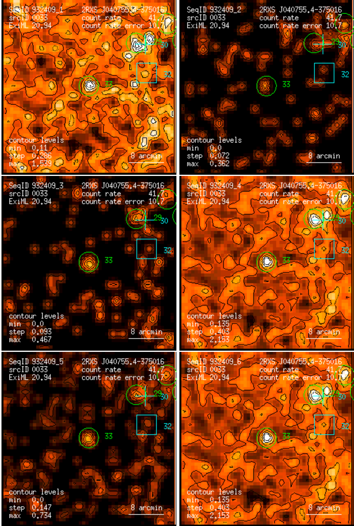
Figure 33: RASS 932409: detection 0033: band rate images, Gaussian filter: (1) PSPC channels 11 – 41, (2) 52 – 90, (3) 91 – 201, (4) 11 – 235, (5) 52 – 201, (6) 11 – 201. Broad band rates in counts/ks. Band rate contour levels in counts/ks/arcmin 2 .
