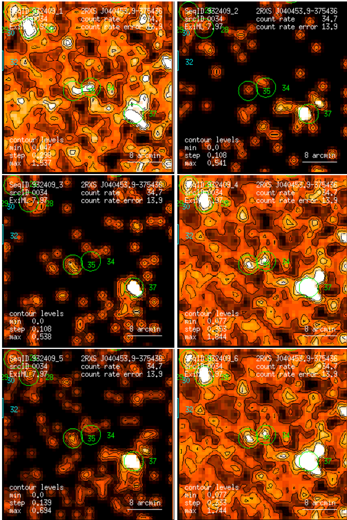
Figure 34: RASS 932409: detection 0034: band rate images, Gaussian filter: (1) PSPC channels 11 – 41, (2) 52 – 90, (3) 91 – 201, (4) 11 – 235, (5) 52 – 201, (6) 11 – 201. Broad band rates in counts/ks. Band rate contour levels in counts/ks/arcmin 2 .
