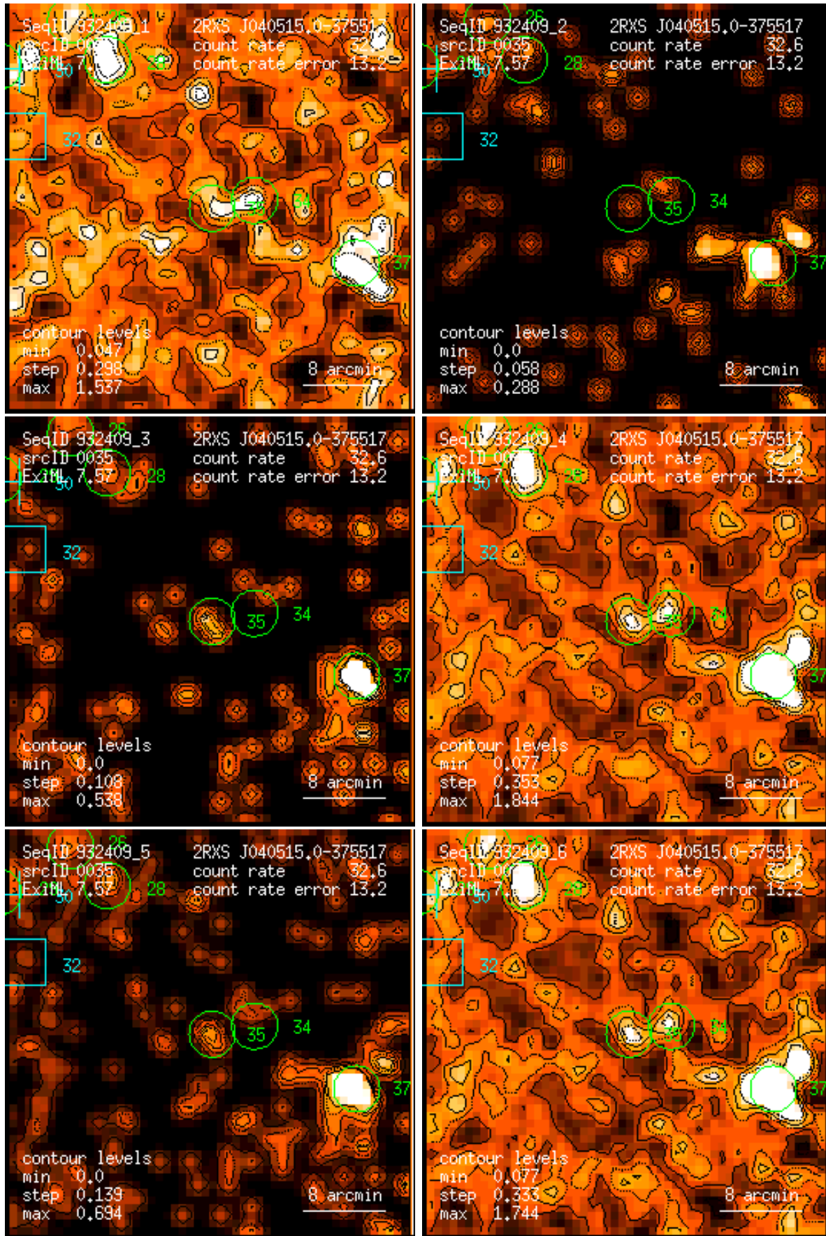
Figure 35: RASS 932409: detection 0035: band rate images, Gaussian filter: (1) PSPC channels 11 – 41, (2) 52 – 90, (3) 91 – 201, (4) 11 – 235, (5) 52 – 201, (6) 11 – 201. Broad band rates in counts/ks. Band rate contour levels in counts/ks/arcmin 2 .
