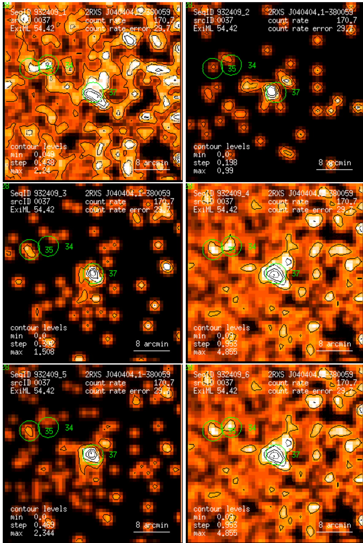
Figure 37: RASS 932409: detection 0037: band rate images, Gaussian filter: (1) PSPC channels 11 – 41, (2) 52 – 90, (3) 91 – 201, (4) 11 – 235, (5) 52 – 201, (6) 11 – 201. Broad band rates in counts/ks. Band rate contour levels in counts/ks/arcmin 2 .
