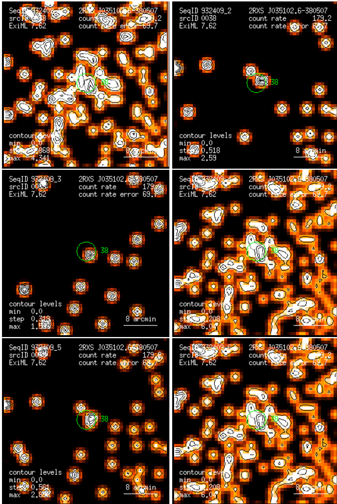
Figure 38: RASS 932409: detection 0038: band rate images, Gaussian filter: (1) PSPC channels 11 – 41, (2) 52 – 90, (3) 91 – 201, (4) 11 – 235, (5) 52 – 201, (6) 11 – 201. Broad band rates in counts/ks. Band rate contour levels in counts/ks/arcmin 2 .
