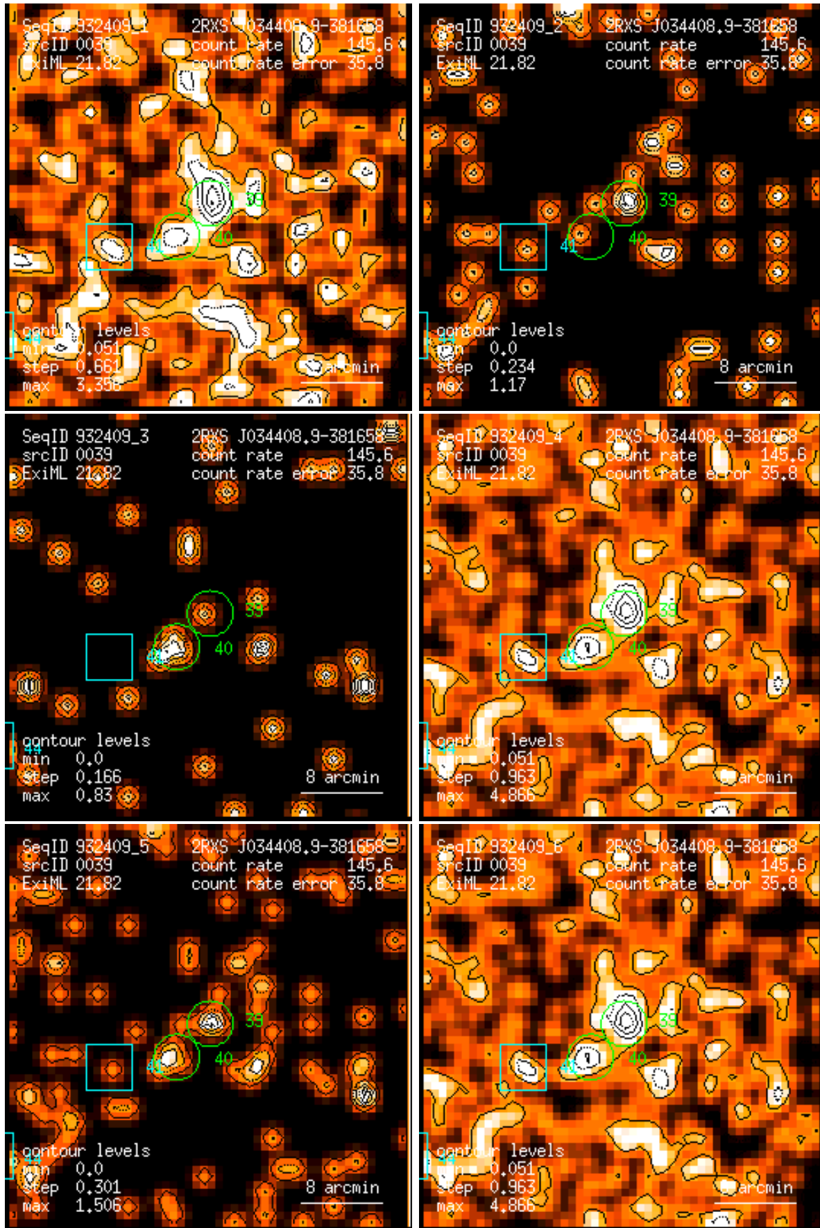
Figure 39: RASS 932409: detection 0039: band rate images, Gaussian filter: (1) PSPC channels 11 – 41, (2) 52 – 90, (3) 91 – 201, (4) 11 – 235, (5) 52 – 201, (6) 11 – 201. Broad band rates in counts/ks. Band rate contour levels in counts/ks/arcmin 2 .
