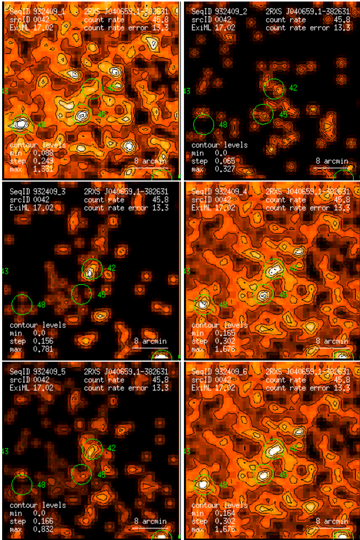
Figure 42: RASS 932409: detection 0042: band rate images, Gaussian filter: (1) PSPC channels 11 – 41, (2) 52 – 90, (3) 91 – 201, (4) 11 – 235, (5) 52 – 201, (6) 11 – 201. Broad band rates in counts/ks. Band rate contour levels in counts/ks/arcmin 2 .
