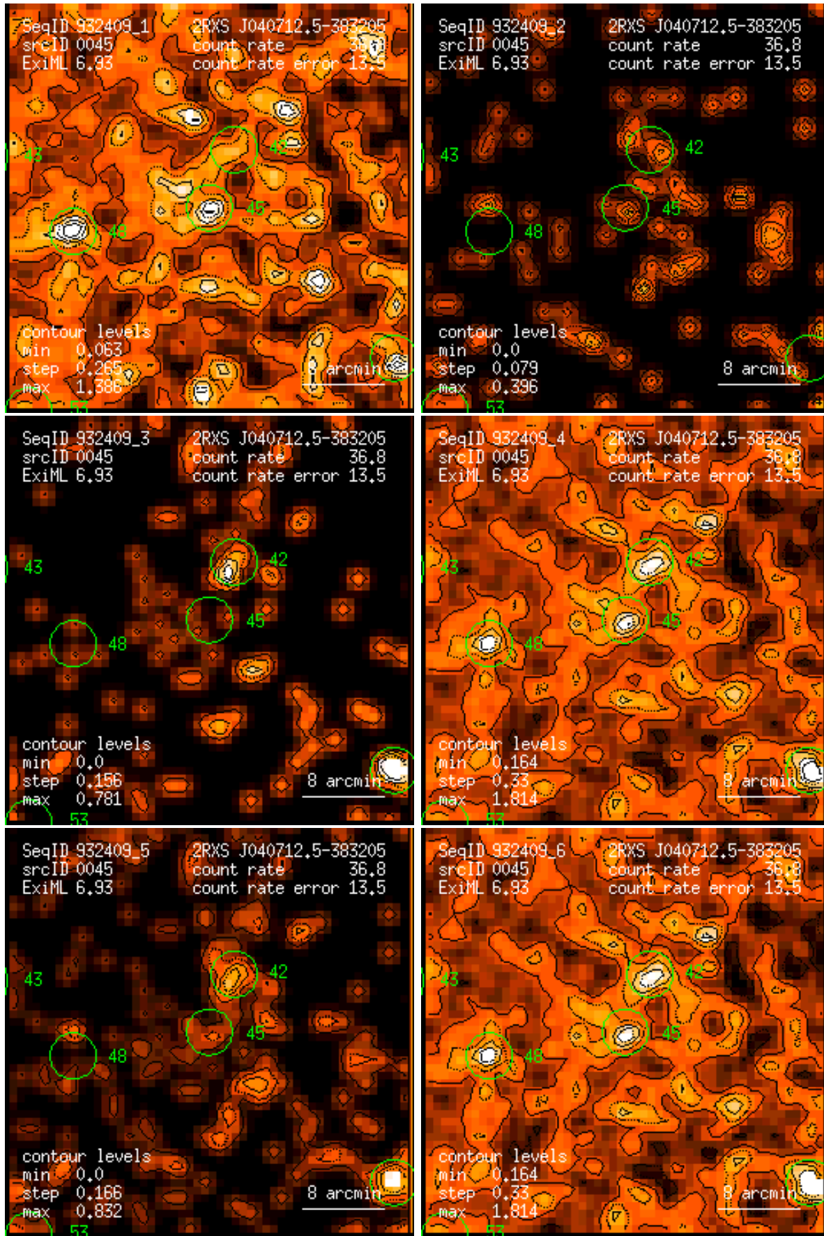
Figure 45: RASS 932409: detection 0045: band rate images, Gaussian filter: (1) PSPC channels 11 – 41, (2) 52 – 90, (3) 91 – 201, (4) 11 – 235, (5) 52 – 201, (6) 11 – 201. Broad band rates in counts/ks. Band rate contour levels in counts/ks/arcmin 2 .
