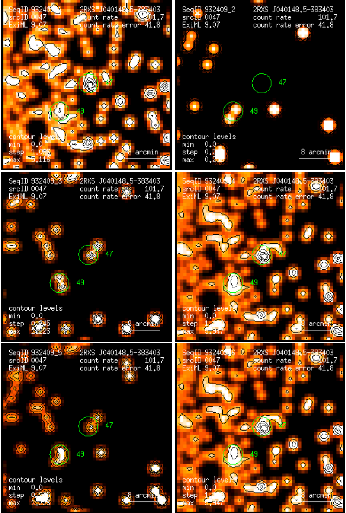
Figure 47: RASS 932409: detection 0047: band rate images, Gaussian filter: (1) PSPC channels 11 – 41, (2) 52 – 90, (3) 91 – 201, (4) 11 – 235, (5) 52 – 201, (6) 11 – 201. Broad band rates in counts/ks. Band rate contour levels in counts/ks/arcmin 2 .
