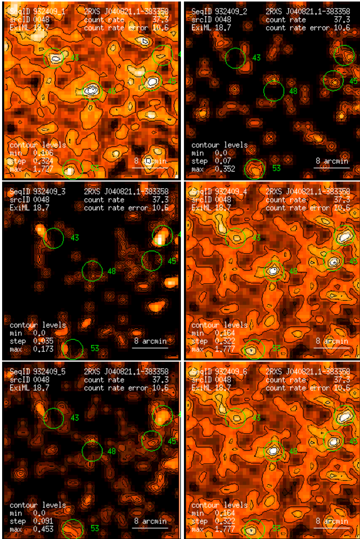
Figure 48: RASS 932409: detection 0048: band rate images, Gaussian filter: (1) PSPC channels 11 – 41, (2) 52 – 90, (3) 91 – 201, (4) 11 – 235, (5) 52 – 201, (6) 11 – 201. Broad band rates in counts/ks. Band rate contour levels in counts/ks/arcmin 2 .
