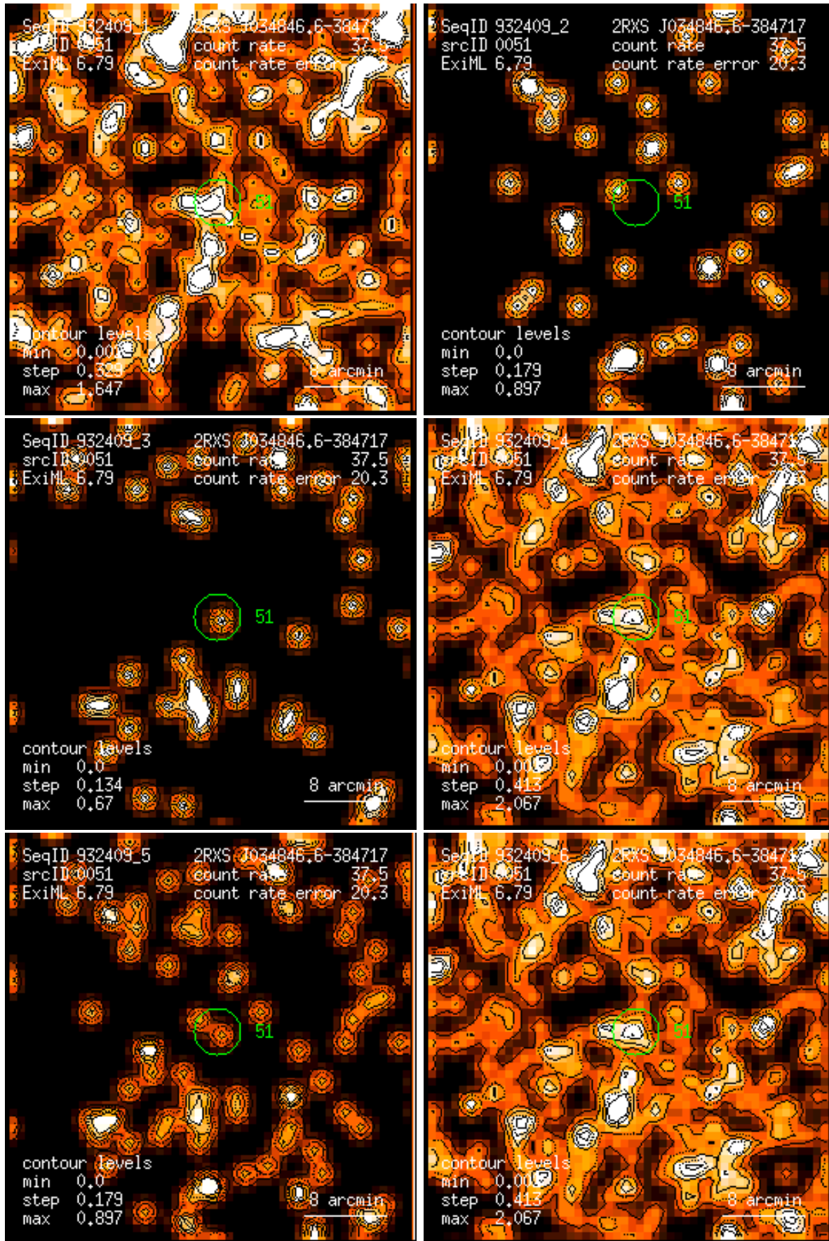
Figure 51: RASS 932409: detection 0051: band rate images, Gaussian filter: (1) PSPC channels 11 – 41, (2) 52 – 90, (3) 91 – 201, (4) 11 – 235, (5) 52 – 201, (6) 11 – 201. Broad band rates in counts/ks. Band rate contour levels in counts/ks/arcmin 2 .
