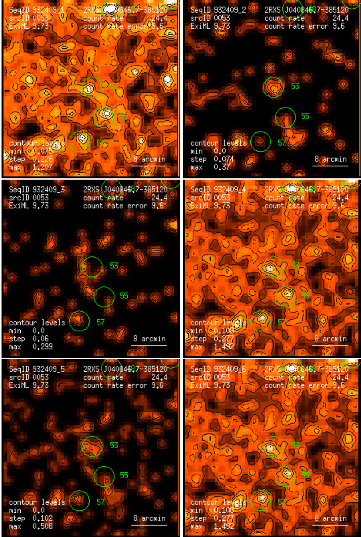
Figure 53: RASS 932409: detection 0053: band rate images, Gaussian filter: (1) PSPC channels 11 – 41, (2) 52 – 90, (3) 91 – 201, (4) 11 – 235, (5) 52 – 201, (6) 11 – 201. Broad band rates in counts/ks. Band rate contour levels in counts/ks/arcmin 2 .
