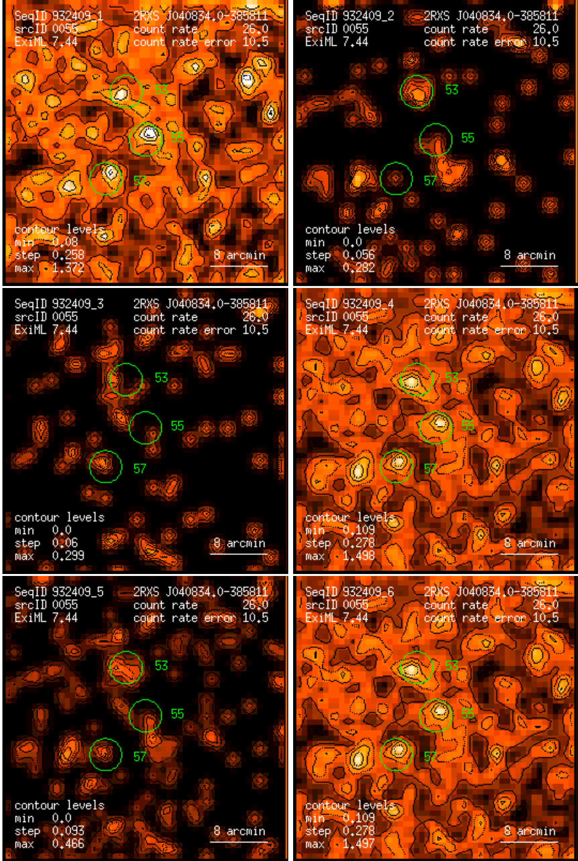
Figure 55: RASS 932409: detection 0055: band rate images, Gaussian filter: (1) PSPC channels 11 – 41, (2) 52 – 90, (3) 91 – 201, (4) 11 – 235, (5) 52 – 201, (6) 11 – 201. Broad band rates in counts/ks. Band rate contour levels in counts/ks/arcmin 2 .
