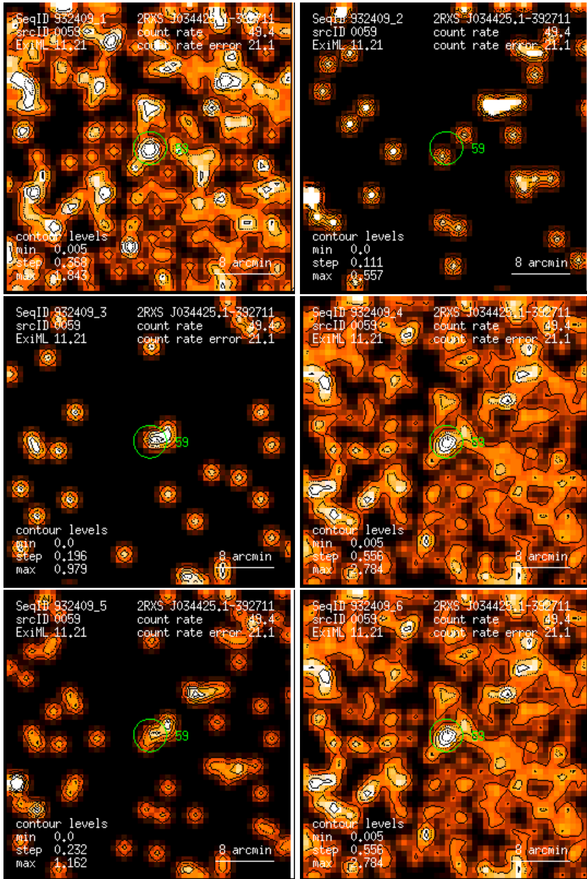
Figure 59: RASS 932409: detection 0059: band rate images, Gaussian filter: (1) PSPC channels 11 – 41, (2) 52 – 90, (3) 91 – 201, (4) 11 – 235, (5) 52 – 201, (6) 11 – 201. Broad band rates in counts/ks. Band rate contour levels in counts/ks/arcmin 2 .
