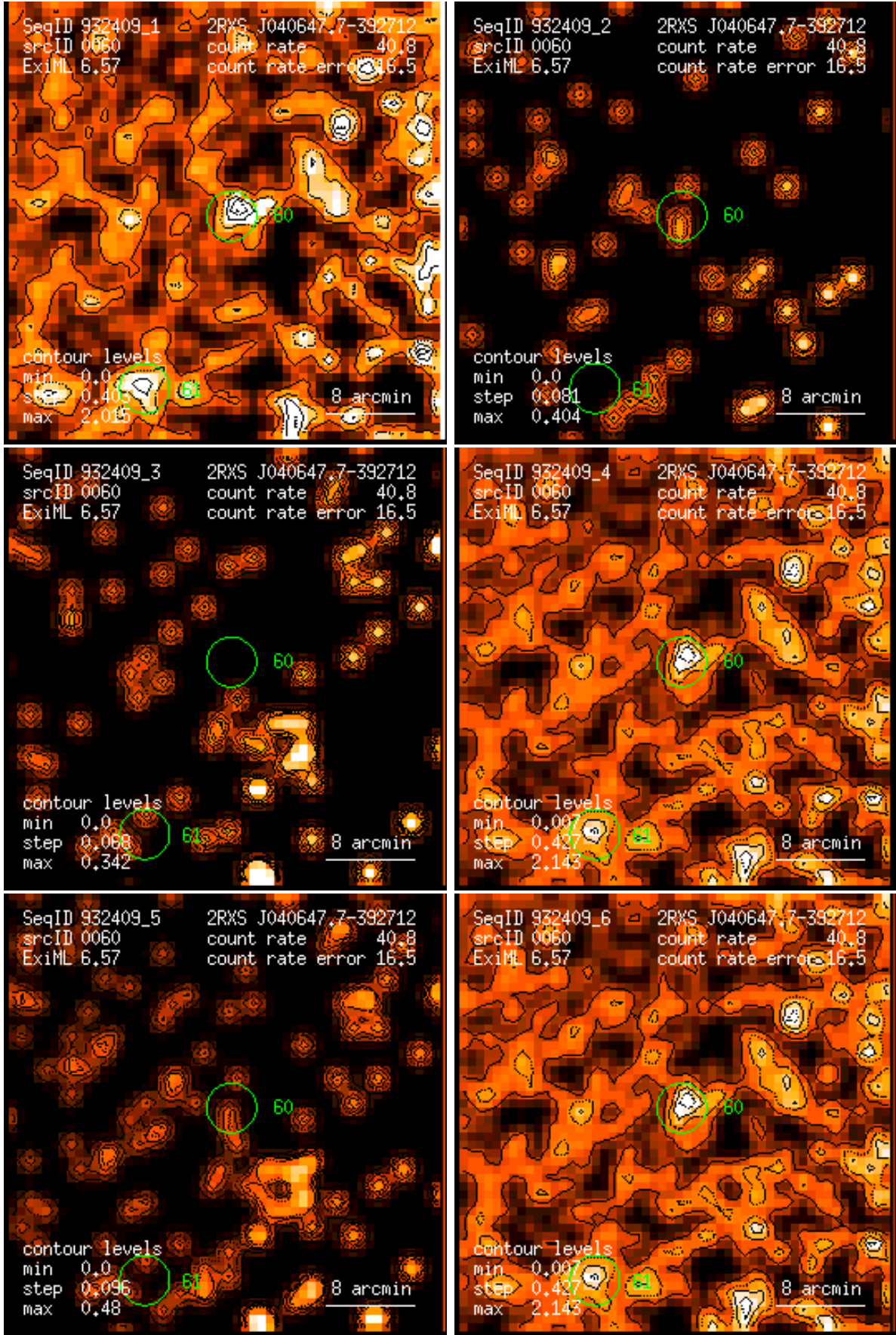
Figure 60: RASS 932409: detection 0060: band rate images, Gaussian filter: (1) PSPC channels 11 – 41, (2) 52 – 90, (3) 91 – 201, (4) 11 – 235, (5) 52 – 201, (6) 11 – 201. Broad band rates in counts/ks. Band rate contour levels in counts/ks/arcmin 2 .
