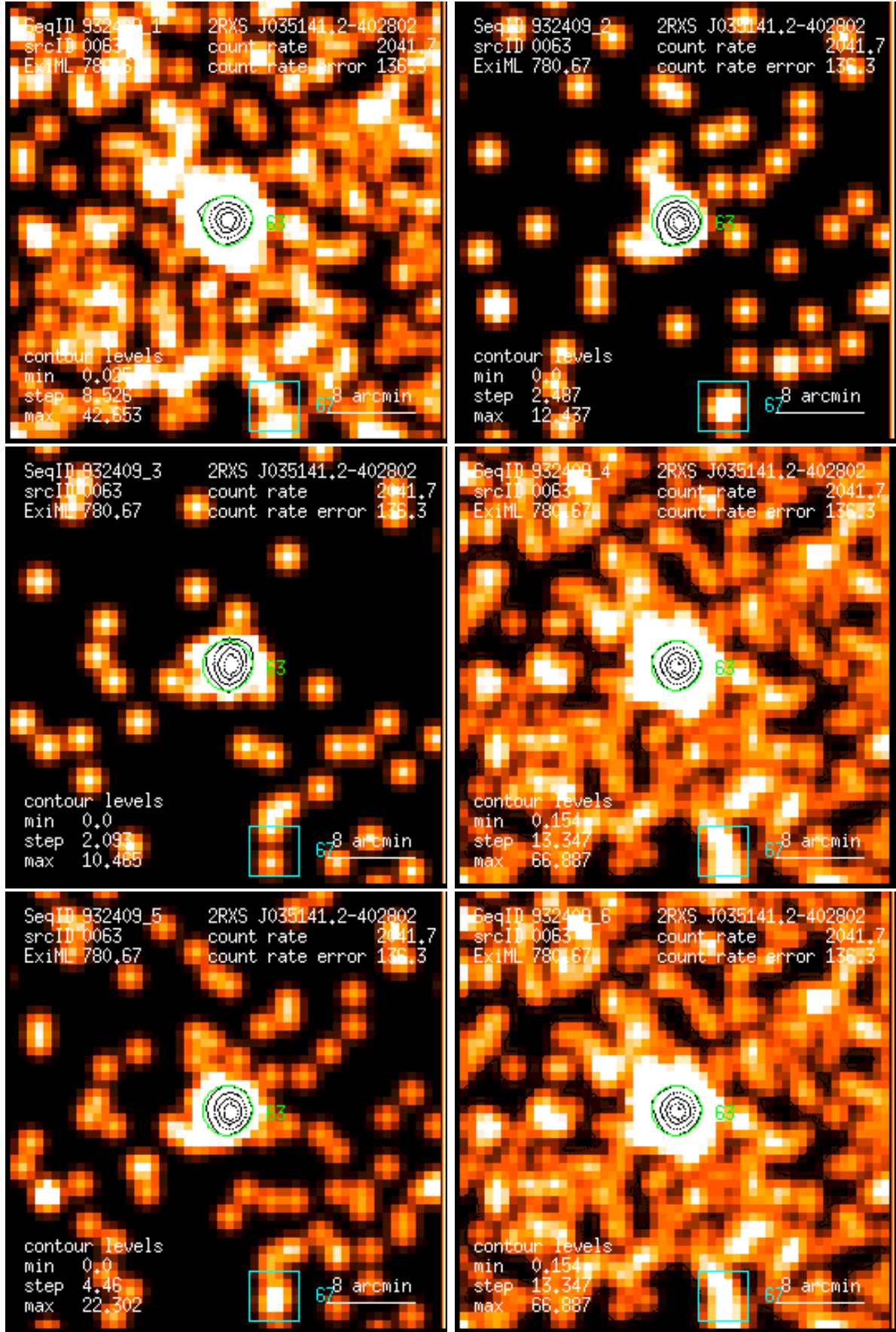
Figure 63: RASS 932409: detection 0063: band rate images, Gaussian filter: (1) PSPC channels 11 – 41, (2) 52 – 90, (3) 91 – 201, (4) 11 – 235, (5) 52 – 201, (6) 11 – 201. Broad band rates in counts/ks. Band rate contour levels in counts/ks/arcmin 2 .
