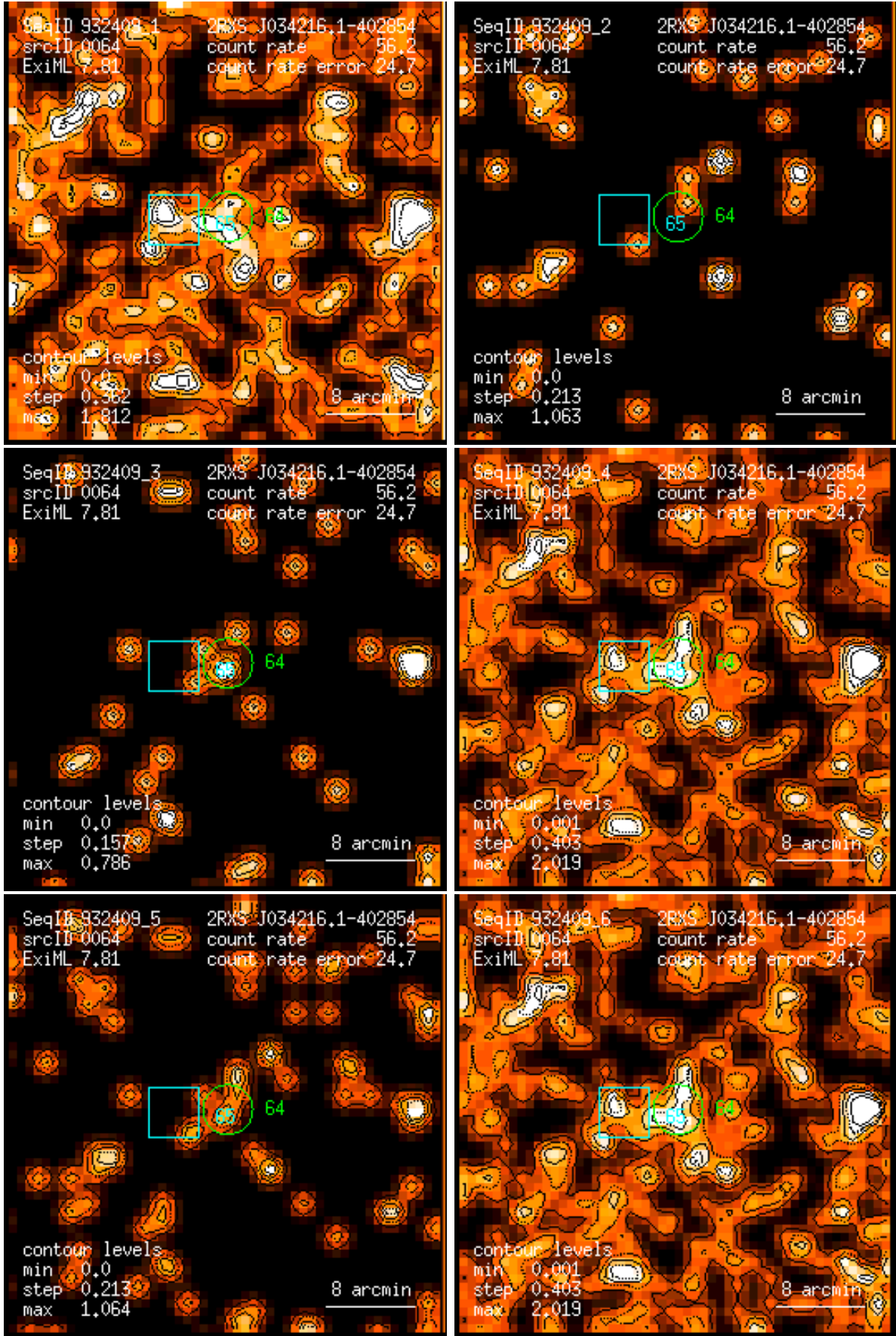
Figure 64: RASS 932409: detection 0064: band rate images, Gaussian filter: (1) PSPC channels 11 – 41, (2) 52 – 90, (3) 91 – 201, (4) 11 – 235, (5) 52 – 201, (6) 11 – 201. Broad band rates in counts/ks. Band rate contour levels in counts/ks/arcmin 2 .
