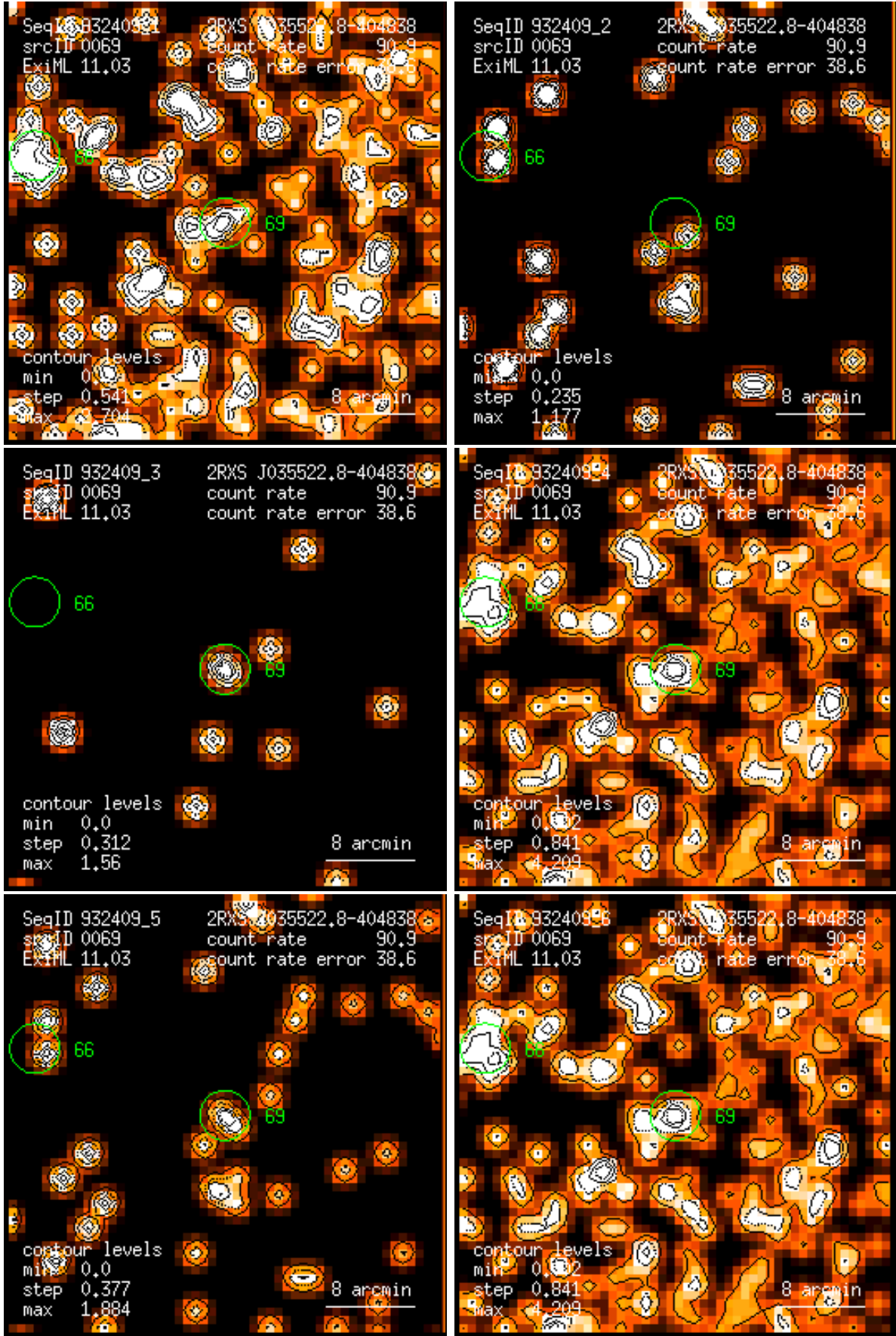
Figure 69: RASS 932409: detection 0069: band rate images, Gaussian filter: (1) PSPC channels 11 – 41, (2) 52 – 90, (3) 91 – 201, (4) 11 – 235, (5) 52 – 201, (6) 11 – 201. Broad band rates in counts/ks. Band rate contour levels in counts/ks/arcmin 2 .
