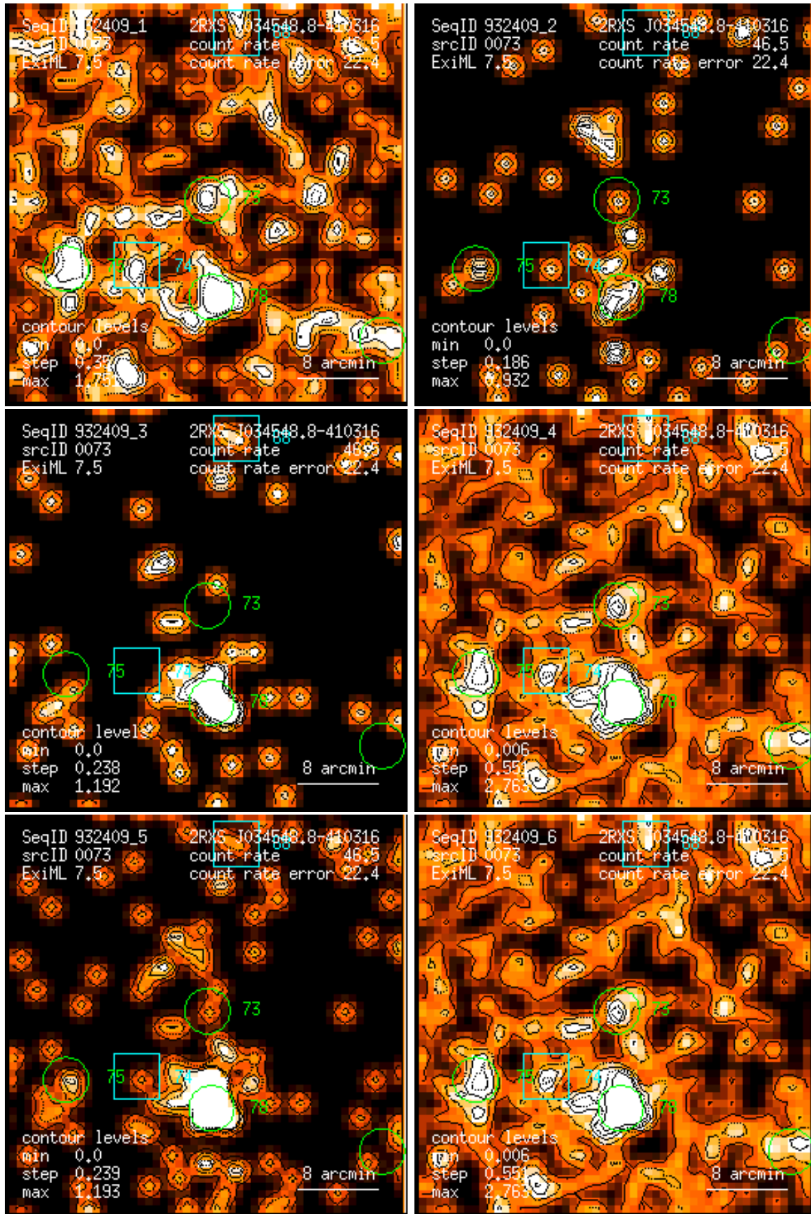
Figure 73: RASS 932409: detection 0073: band rate images, Gaussian filter: (1) PSPC channels 11 – 41, (2) 52 – 90, (3) 91 – 201, (4) 11 – 235, (5) 52 – 201, (6) 11 – 201. Broad band rates in counts/ks. Band rate contour levels in counts/ks/arcmin 2 .
