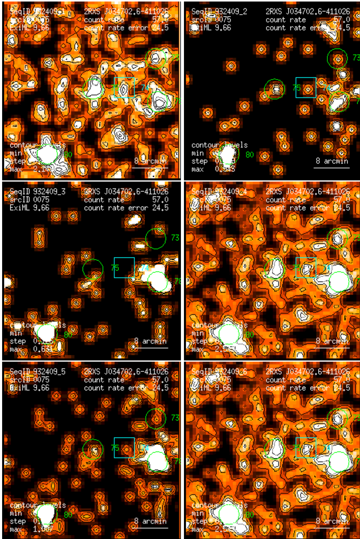
Figure 75: RASS 932409: detection 0075: band rate images, Gaussian filter: (1) PSPC channels 11 – 41, (2) 52 – 90, (3) 91 – 201, (4) 11 – 235, (5) 52 – 201, (6) 11 – 201. Broad band rates in counts/ks. Band rate contour levels in counts/ks/arcmin 2 .
