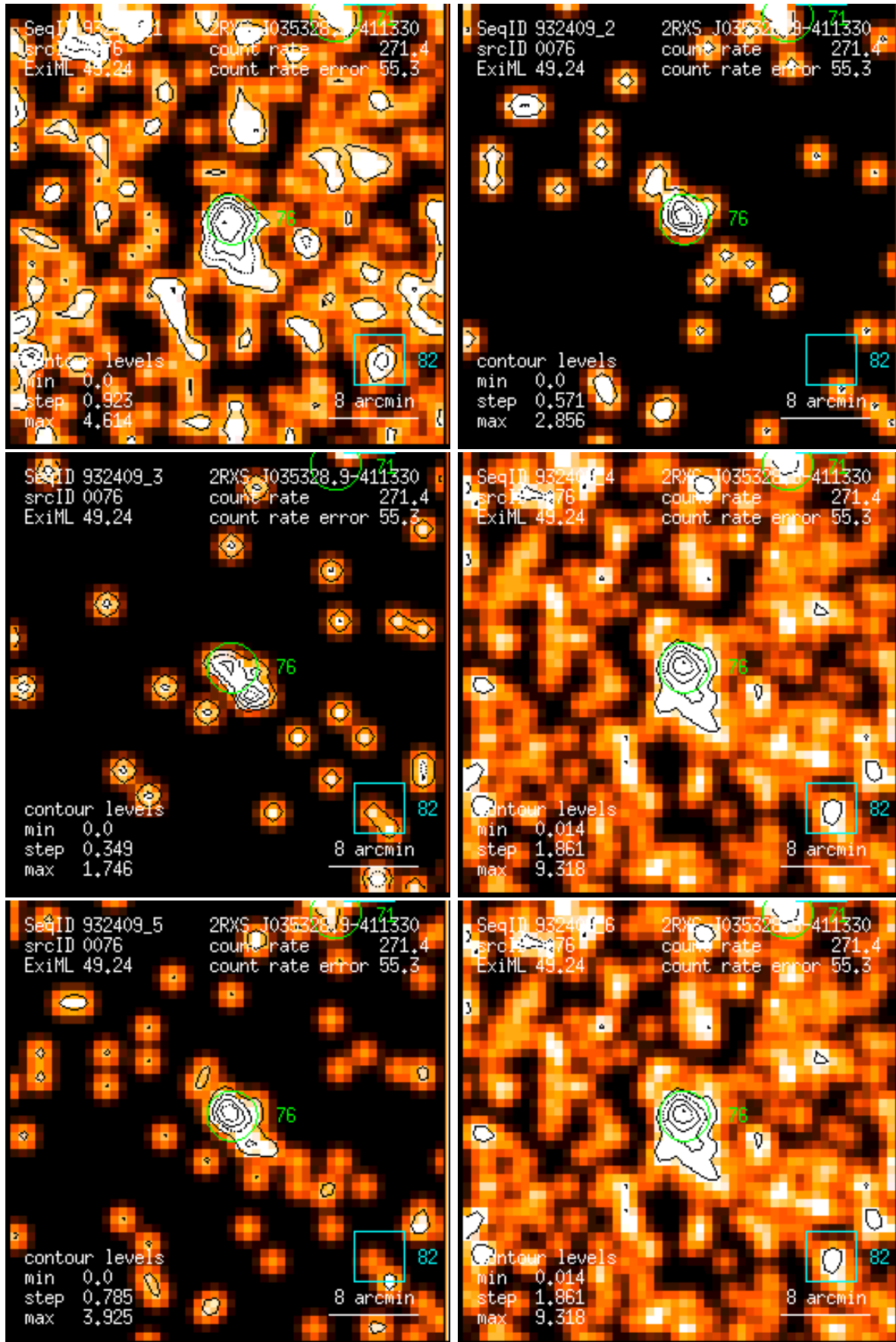
Figure 76: RASS 932409: detection 0076: band rate images, Gaussian filter: (1) PSPC channels 11 – 41, (2) 52 – 90, (3) 91 – 201, (4) 11 – 235, (5) 52 – 201, (6) 11 – 201. Broad band rates in counts/ks. Band rate contour levels in counts/ks/arcmin 2 .
