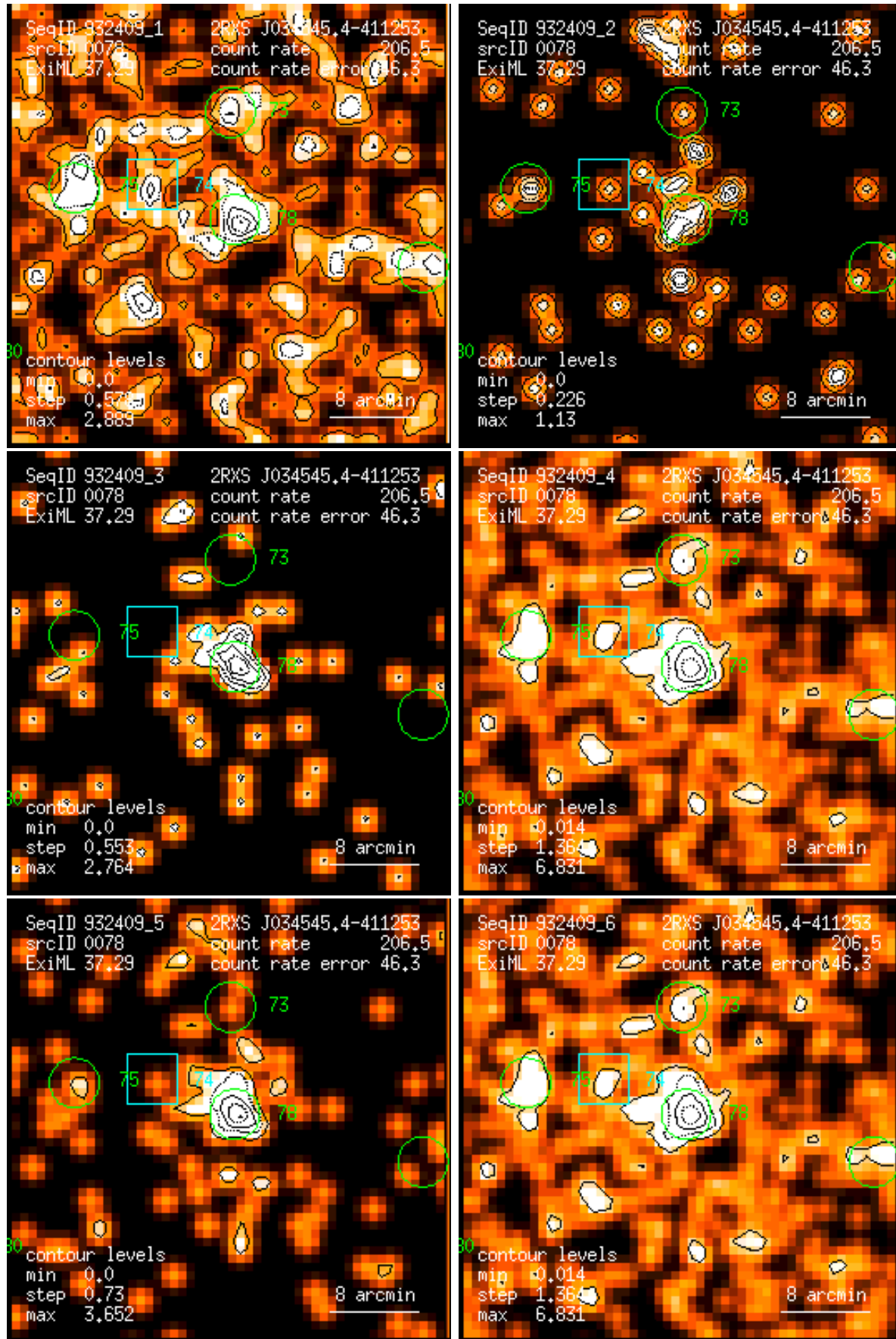
Figure 78: RASS 932409: detection 0078: band rate images, Gaussian filter: (1) PSPC channels 11 – 41, (2) 52 – 90, (3) 91 – 201, (4) 11 – 235, (5) 52 – 201, (6) 11 – 201. Broad band rates in counts/ks. Band rate contour levels in counts/ks/arcmin 2 .
