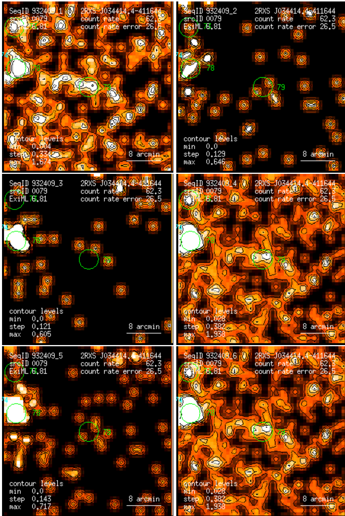
Figure 79: RASS 932409: detection 0079: band rate images, Gaussian filter: (1) PSPC channels 11 – 41, (2) 52 – 90, (3) 91 – 201, (4) 11 – 235, (5) 52 – 201, (6) 11 – 201. Broad band rates in counts/ks. Band rate contour levels in counts/ks/arcmin 2 .
