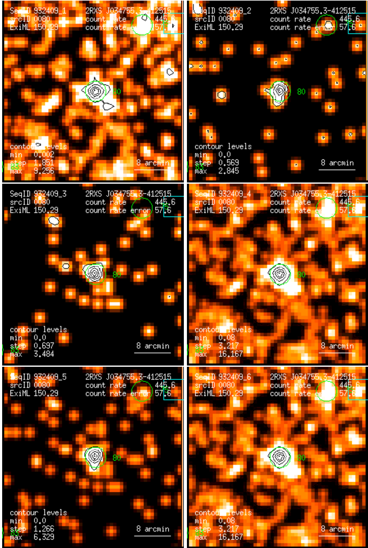
Figure 80: RASS 932409: detection 0080: band rate images, Gaussian filter: (1) PSPC channels 11 – 41, (2) 52 – 90, (3) 91 – 201, (4) 11 – 235, (5) 52 – 201, (6) 11 – 201. Broad band rates in counts/ks. Band rate contour levels in counts/ks/arcmin 2 .
