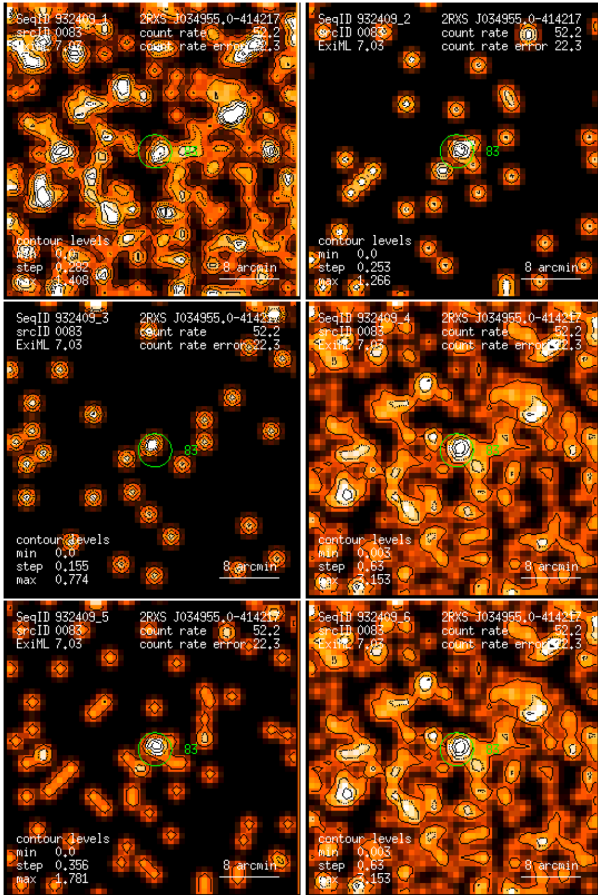
Figure 83: RASS 932409: detection 0083: band rate images, Gaussian filter: (1) PSPC channels 11 – 41, (2) 52 – 90, (3) 91 – 201, (4) 11 – 235, (5) 52 – 201, (6) 11 – 201. Broad band rates in counts/ks. Band rate contour levels in counts/ks/arcmin 2 .
