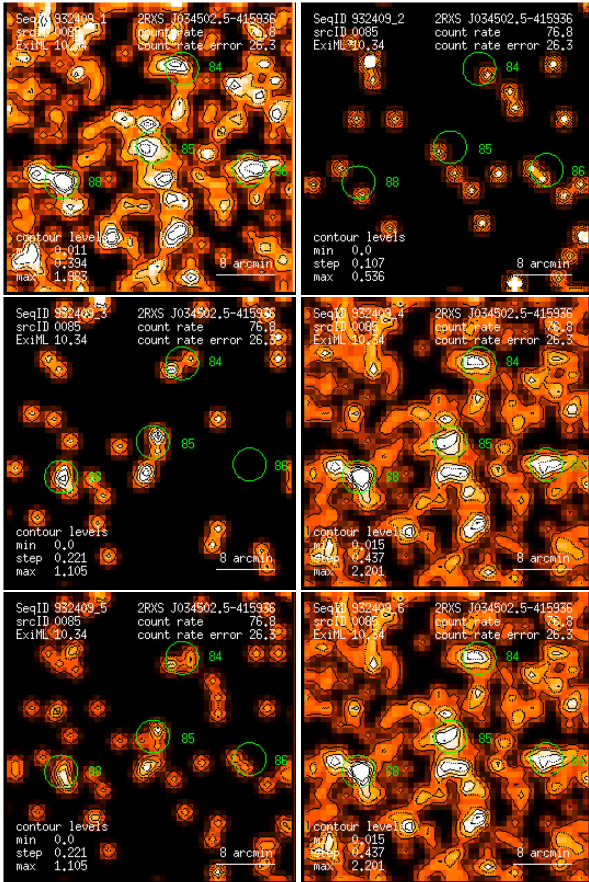
Figure 85: RASS 932409: detection 0085: band rate images, Gaussian filter: (1) PSPC channels 11 – 41, (2) 52 – 90, (3) 91 – 201, (4) 11 – 235, (5) 52 – 201, (6) 11 – 201. Broad band rates in counts/ks. Band rate contour levels in counts/ks/arcmin 2 .
