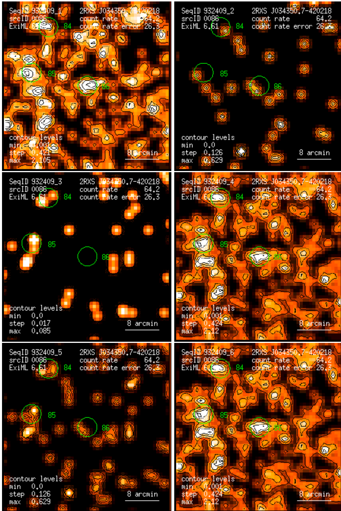
Figure 86: RASS 932409: detection 0086: band rate images, Gaussian filter: (1) PSPC channels 11 – 41, (2) 52 – 90, (3) 91 – 201, (4) 11 – 235, (5) 52 – 201, (6) 11 – 201. Broad band rates in counts/ks. Band rate contour levels in counts/ks/arcmin 2 .
