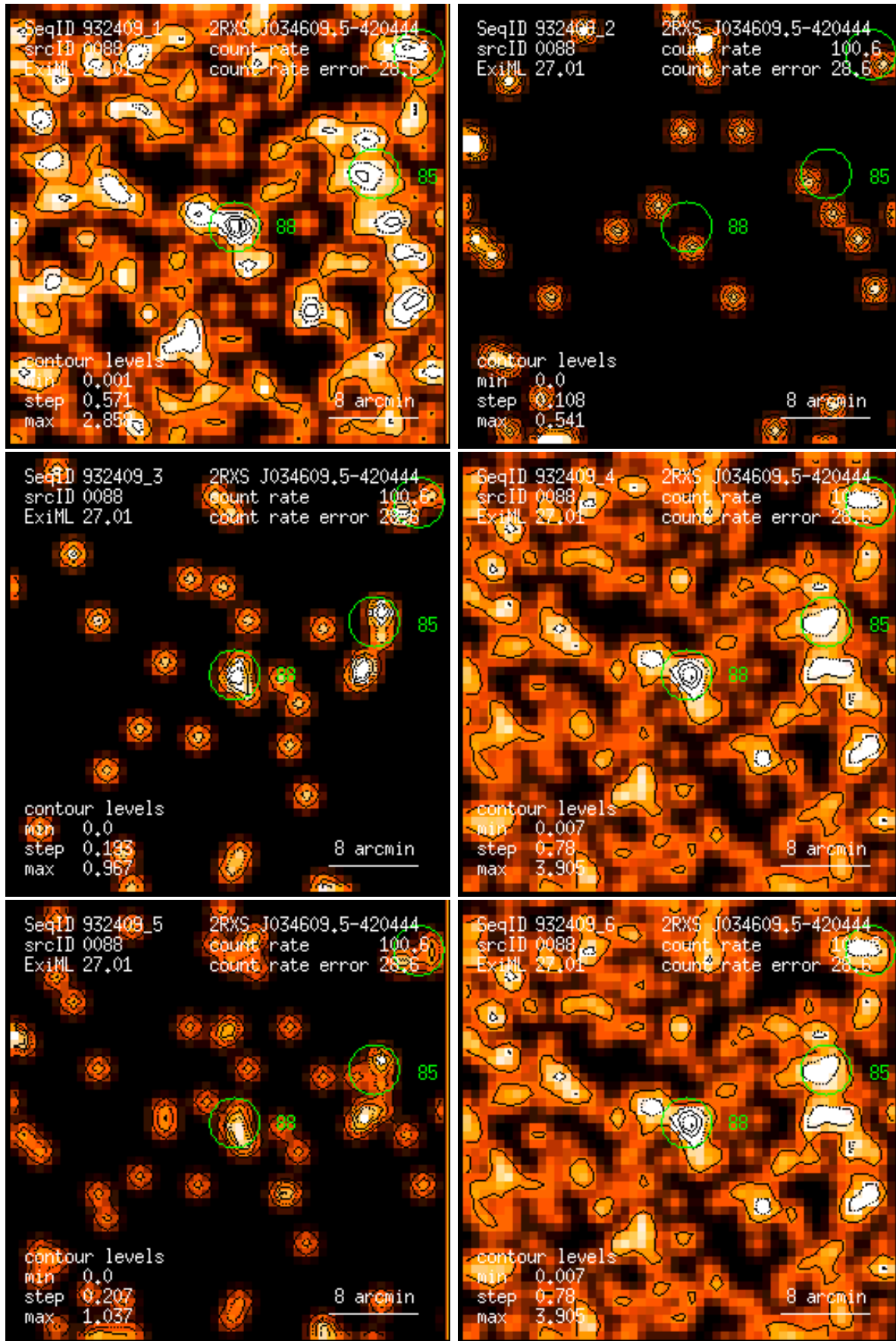
Figure 88: RASS 932409: detection 0088: band rate images, Gaussian filter: (1) PSPC channels 11 – 41, (2) 52 – 90, (3) 91 – 201, (4) 11 – 235, (5) 52 – 201, (6) 11 – 201. Broad band rates in counts/ks. Band rate contour levels in counts/ks/arcmin 2 .
