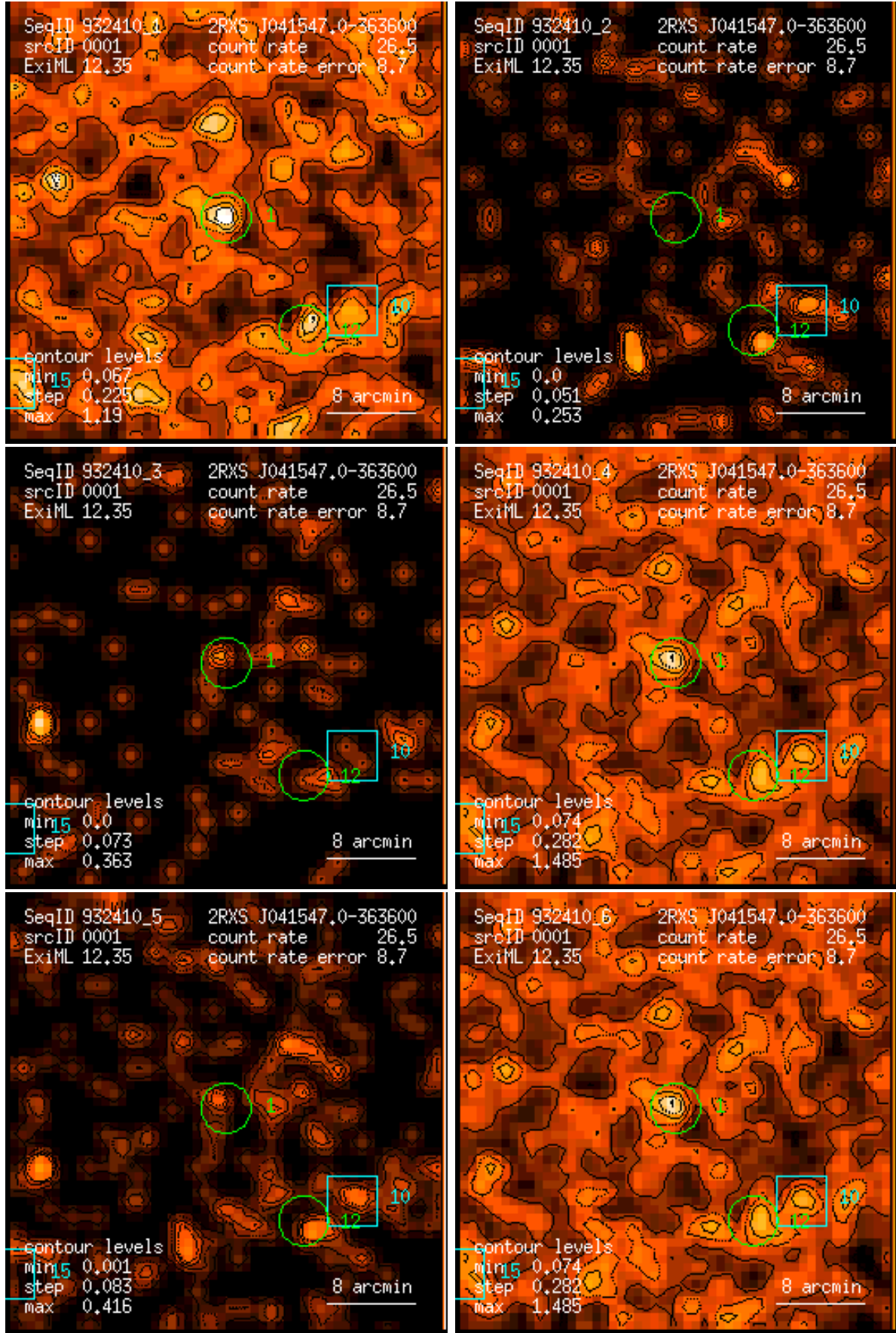
Figure 1: RASS 932410: detection 0001: band rate images, Gaussian filter: (1) PSPC channels 11 – 41, (2) 52 – 90, (3) 91 – 201, (4) 11 – 235, (5) 52 – 201, (6) 11 – 201. Broad band rates in counts/ks. Band rate contour levels in counts/ks/arcmin 2 .
