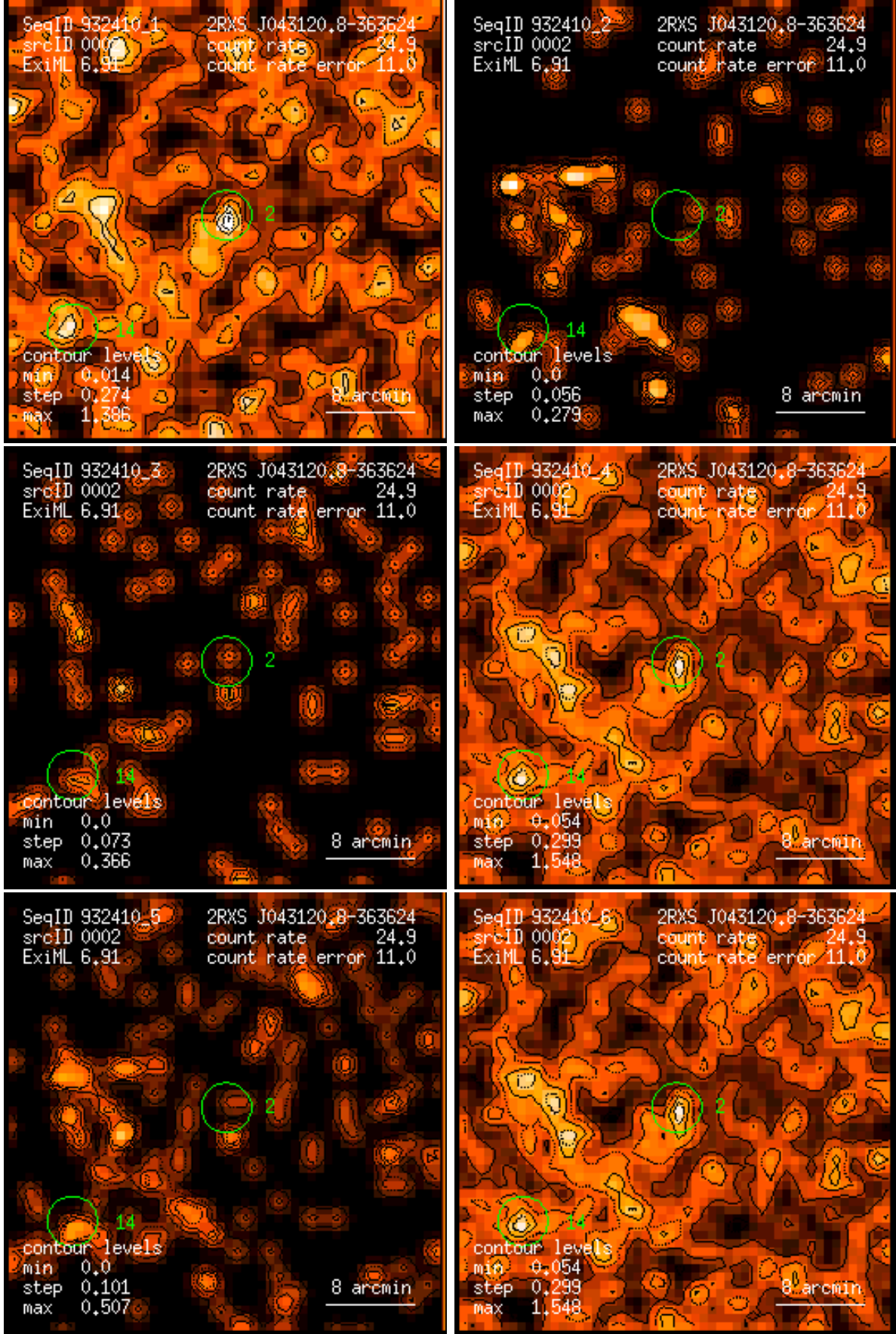
Figure 2: RASS 932410: detection 0002: band rate images, Gaussian filter: (1) PSPC channels 11 – 41, (2) 52 – 90, (3) 91 – 201, (4) 11 – 235, (5) 52 – 201, (6) 11 – 201. Broad band rates in counts/ks. Band rate contour levels in counts/ks/arcmin 2 .
