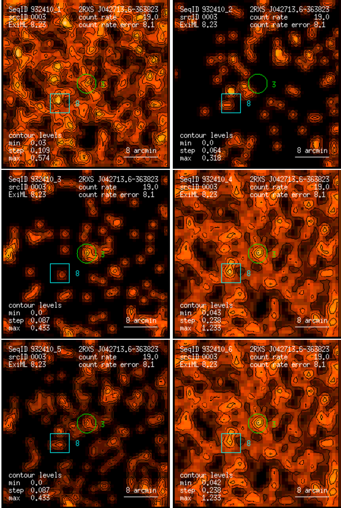
Figure 3: RASS 932410: detection 0003: band rate images, Gaussian filter: (1) PSPC channels 11 – 41, (2) 52 – 90, (3) 91 – 201, (4) 11 – 235, (5) 52 – 201, (6) 11 – 201. Broad band rates in counts/ks. Band rate contour levels in counts/ks/arcmin 2 .
