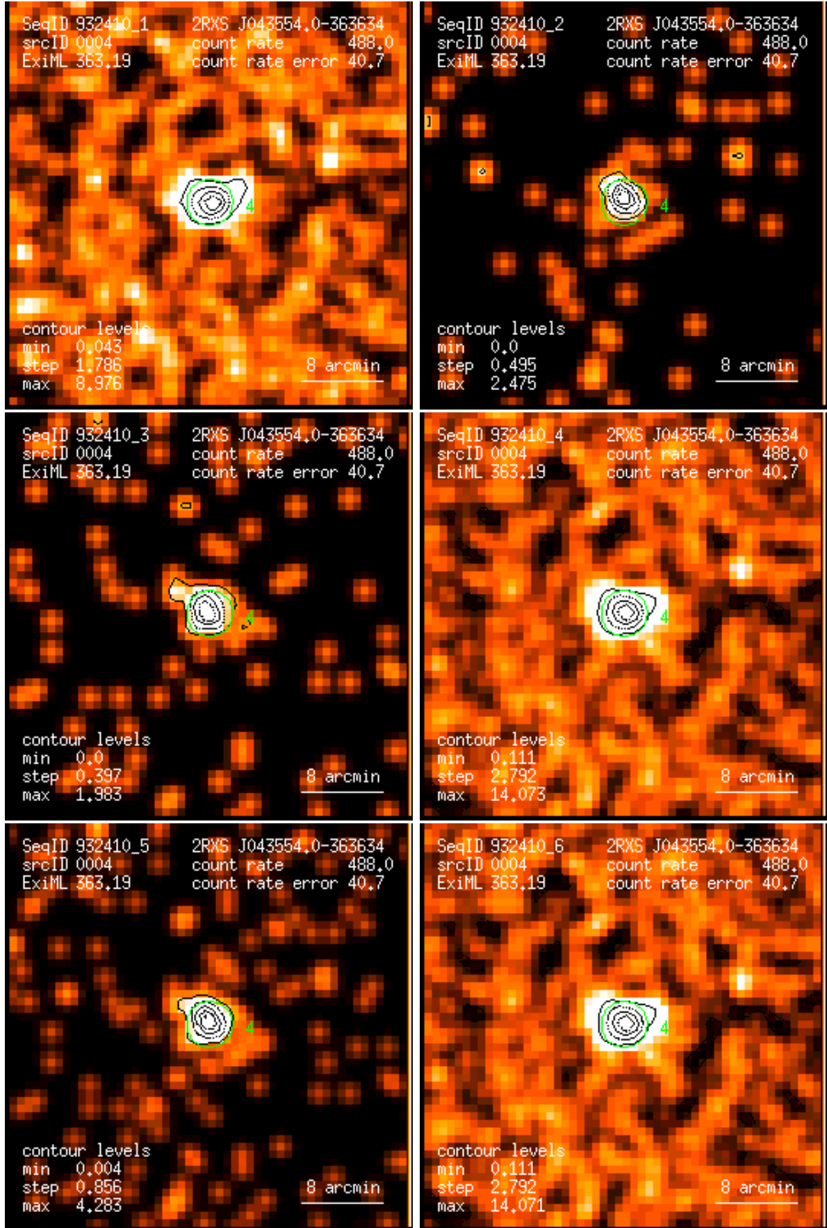
Figure 4: RASS 932410: detection 0004: band rate images, Gaussian filter: (1) PSPC channels 11 – 41, (2) 52 – 90, (3) 91 – 201, (4) 11 – 235, (5) 52 – 201, (6) 11 – 201. Broad band rates in counts/ks. Band rate contour levels in counts/ks/arcmin 2 .
