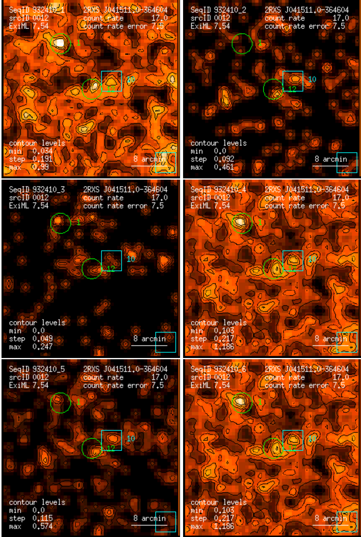
Figure 12: RASS 932410: detection 0012: band rate images, Gaussian filter: (1) PSPC channels 11 – 41, (2) 52 – 90, (3) 91 – 201, (4) 11 – 235, (5) 52 – 201, (6) 11 – 201. Broad band rates in counts/ks. Band rate contour levels in counts/ks/arcmin 2 .
