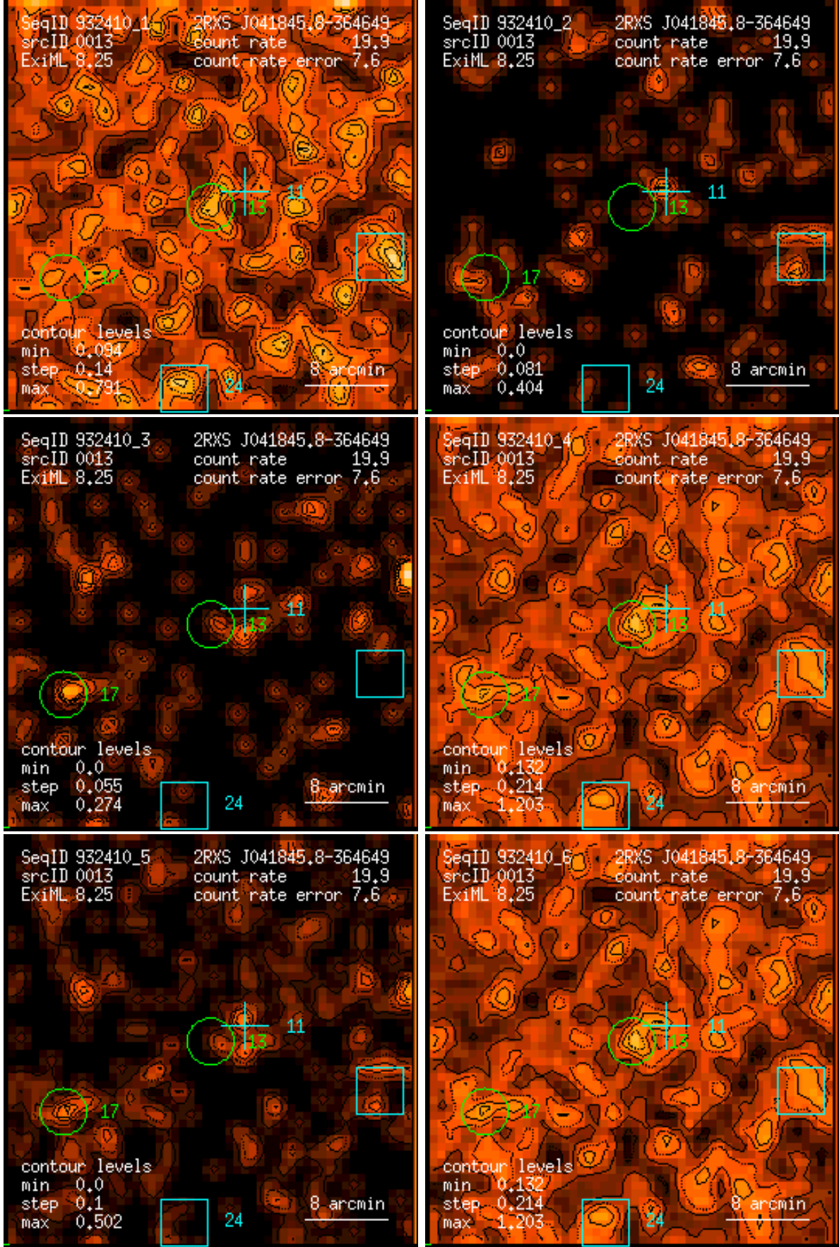
Figure 13: RASS 932410: detection 0013: band rate images, Gaussian filter: (1) PSPC channels 11 – 41, (2) 52 – 90, (3) 91 – 201, (4) 11 – 235, (5) 52 – 201, (6) 11 – 201. Broad band rates in counts/ks. Band rate contour levels in counts/ks/arcmin 2 .
